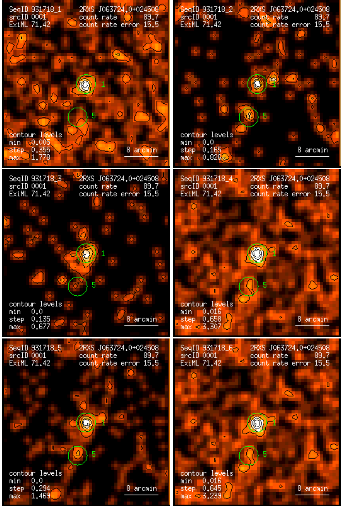
Figure 1: RASS 931718: detection 0001: band rate images, Gaussian filter: (1) PSPC channels 11 – 41, (2) 52 – 90, (3) 91 – 201, (4) 11 – 235, (5) 52 – 201, (6) 11 – 201. Broad band rates in counts/ks. Band rate contour levels in counts/ks/arcmin 2 .
