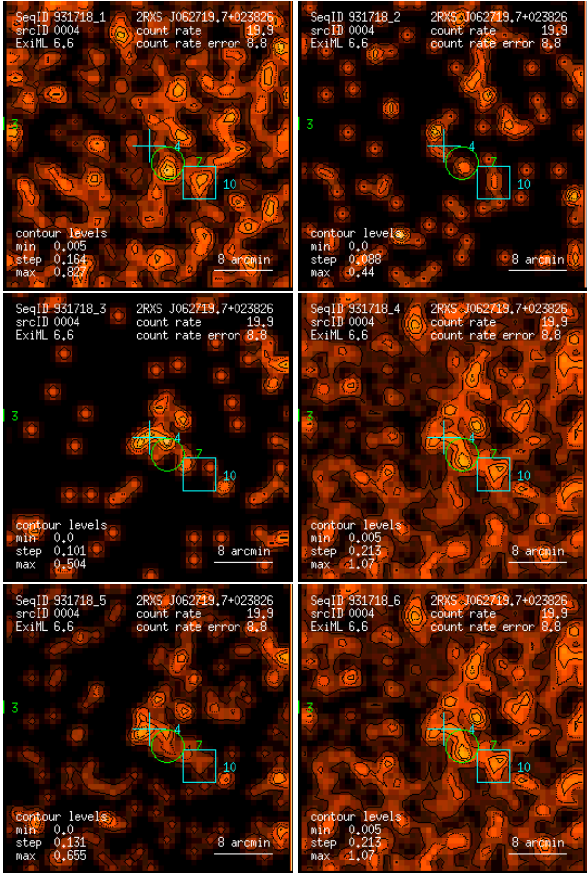
Figure 4: RASS 931718: detection 0004: band rate images, Gaussian filter: (1) PSPC channels 11 – 41, (2) 52 – 90, (3) 91 – 201, (4) 11 – 235, (5) 52 – 201, (6) 11 – 201. Broad band rates in counts/ks. Band rate contour levels in counts/ks/arcmin 2 .
