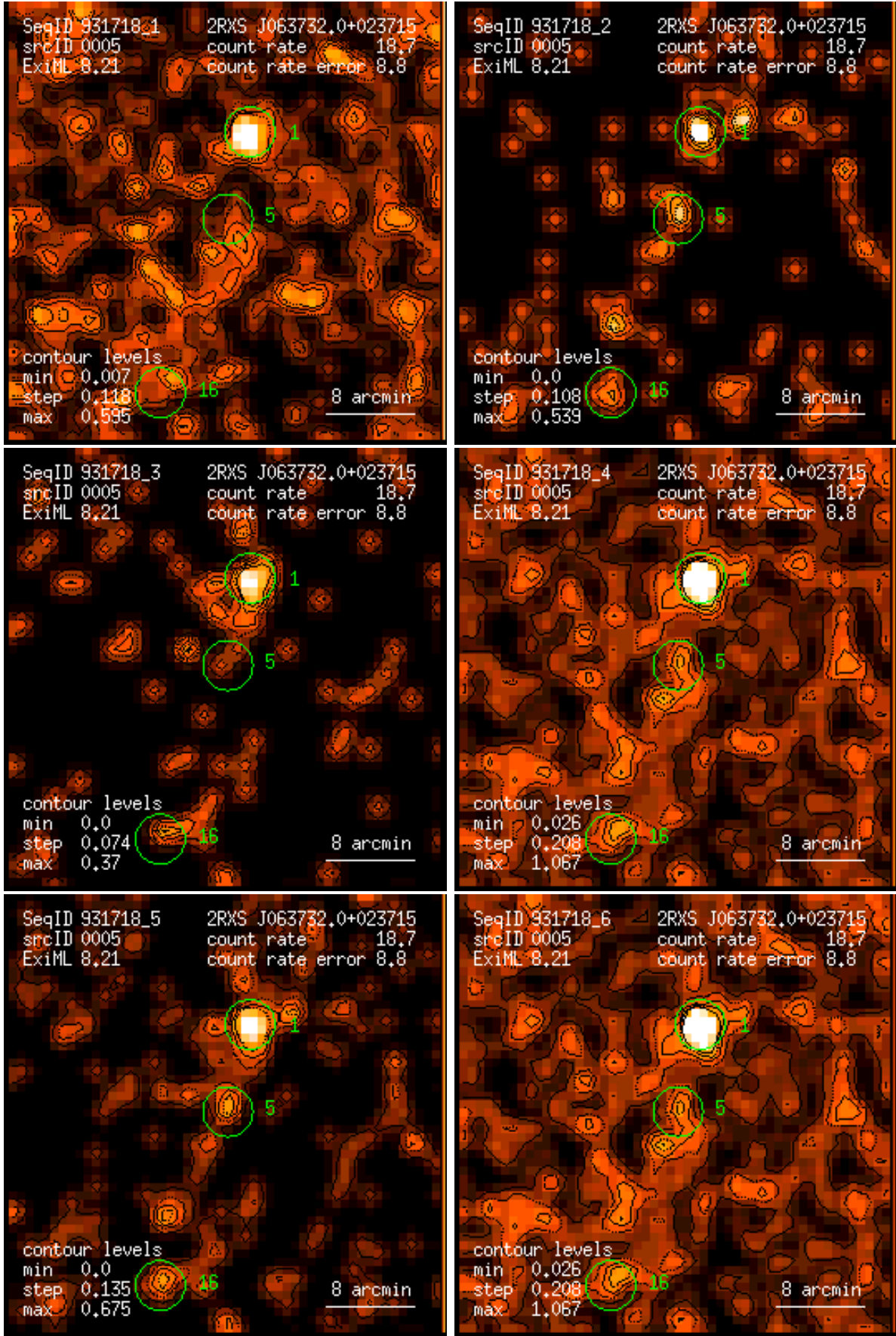
Figure 5: RASS 931718: detection 0005: band rate images, Gaussian filter: (1) PSPC channels 11 – 41, (2) 52 – 90, (3) 91 – 201, (4) 11 – 235, (5) 52 – 201, (6) 11 – 201. Broad band rates in counts/ks. Band rate contour levels in counts/ks/arcmin 2 .
