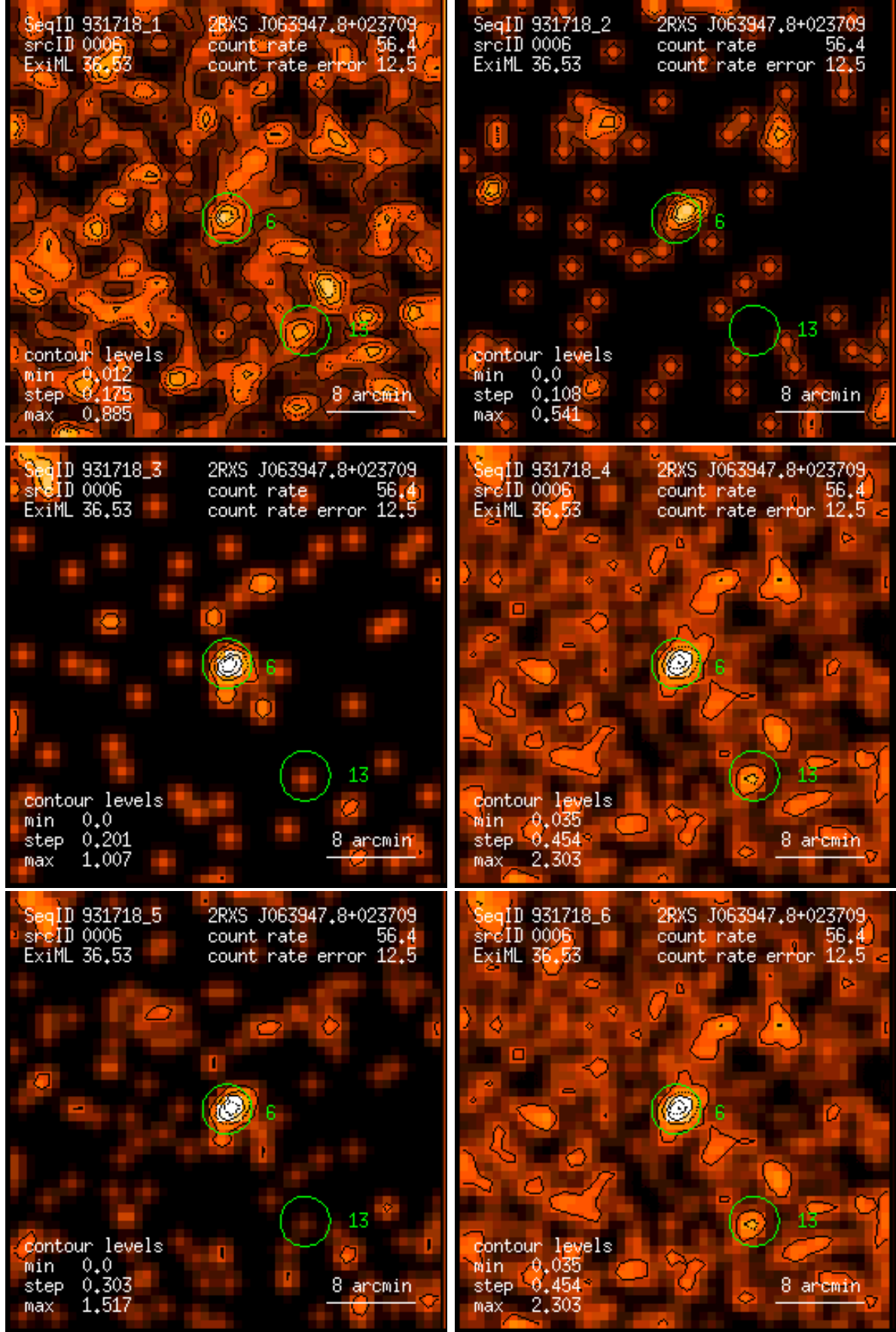
Figure 6: RASS 931718: detection 0006: band rate images, Gaussian filter: (1) PSPC channels 11 – 41, (2) 52 – 90, (3) 91 – 201, (4) 11 – 235, (5) 52 – 201, (6) 11 – 201. Broad band rates in counts/ks. Band rate contour levels in counts/ks/arcmin 2 .
