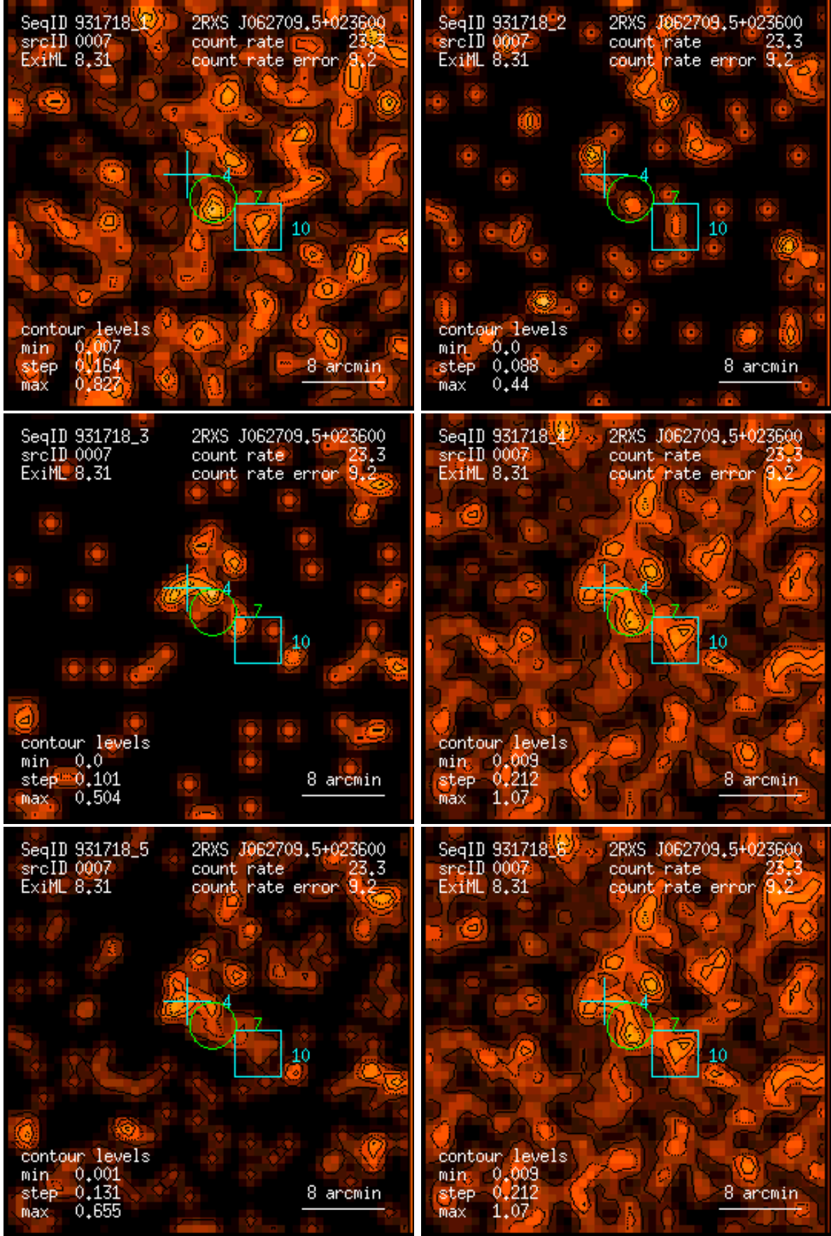
Figure 7: RASS 931718: detection 0007: band rate images, Gaussian filter: (1) PSPC channels 11 – 41, (2) 52 – 90, (3) 91 – 201, (4) 11 – 235, (5) 52 – 201, (6) 11 – 201. Broad band rates in counts/ks. Band rate contour levels in counts/ks/arcmin 2 .
