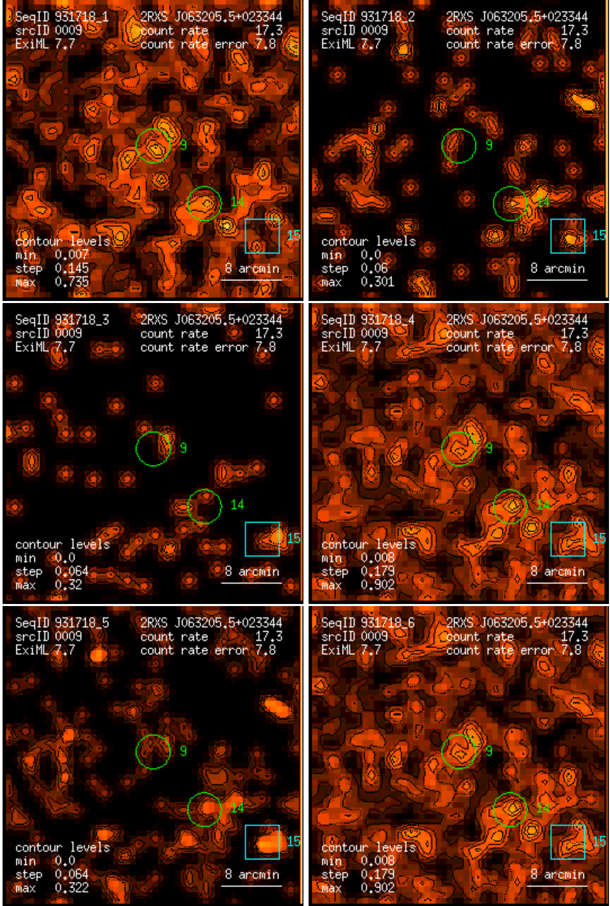
Figure 9: RASS 931718: detection 0009: band rate images, Gaussian filter: (1) PSPC channels 11 – 41, (2) 52 – 90, (3) 91 – 201, (4) 11 – 235, (5) 52 – 201, (6) 11 – 201. Broad band rates in counts/ks. Band rate contour levels in counts/ks/arcmin 2 .
