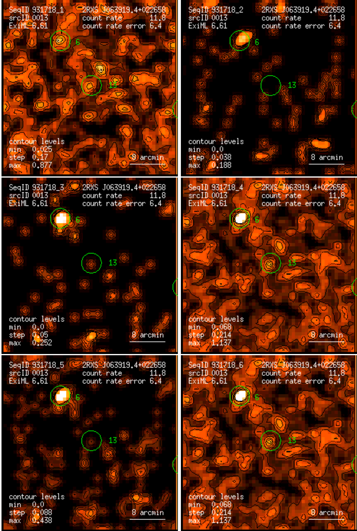
Figure 13: RASS 931718: detection 0013: band rate images, Gaussian filter: (1) PSPC channels 11 – 41, (2) 52 – 90, (3) 91 – 201, (4) 11 – 235, (5) 52 – 201, (6) 11 – 201. Broad band rates in counts/ks. Band rate contour levels in counts/ks/arcmin 2 .
