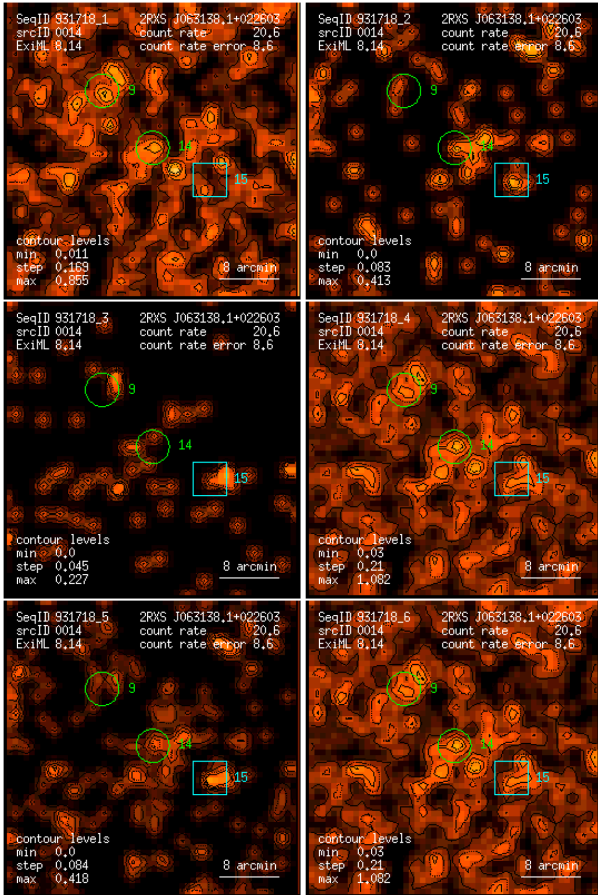
Figure 14: RASS 931718: detection 0014: band rate images, Gaussian filter: (1) PSPC channels 11 – 41, (2) 52 – 90, (3) 91 – 201, (4) 11 – 235, (5) 52 – 201, (6) 11 – 201. Broad band rates in counts/ks. Band rate contour levels in counts/ks/arcmin 2 .
