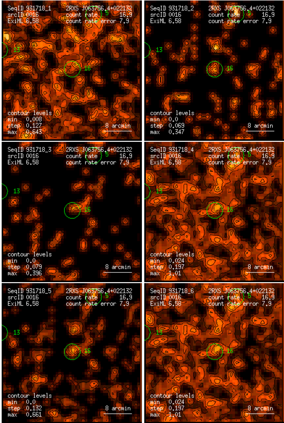
Figure 16: RASS 931718: detection 0016: band rate images, Gaussian filter: (1) PSPC channels 11 – 41, (2) 52 – 90, (3) 91 – 201, (4) 11 – 235, (5) 52 – 201, (6) 11 – 201. Broad band rates in counts/ks. Band rate contour levels in counts/ks/arcmin 2 .
