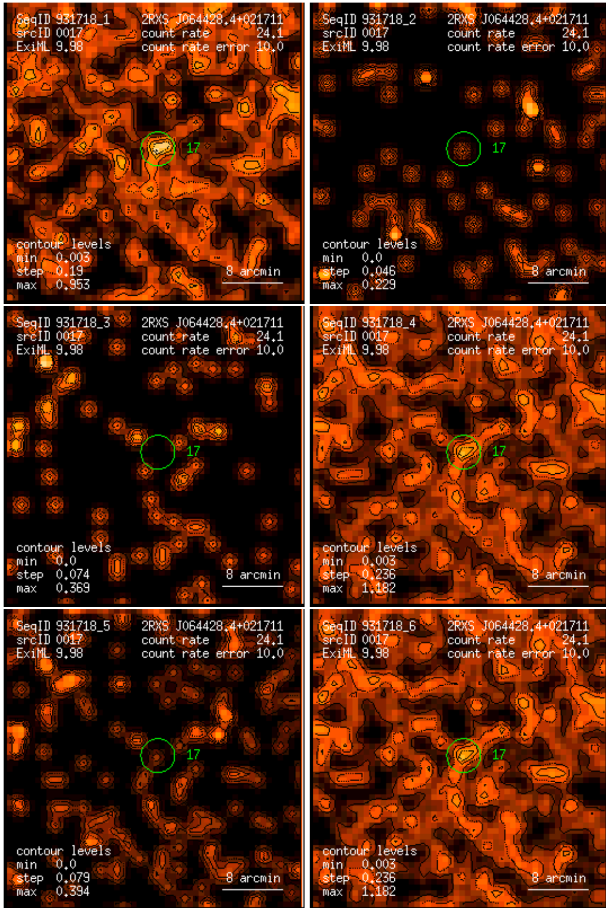
Figure 17: RASS 931718: detection 0017: band rate images, Gaussian filter: (1) PSPC channels 11 – 41, (2) 52 – 90, (3) 91 – 201, (4) 11 – 235, (5) 52 – 201, (6) 11 – 201. Broad band rates in counts/ks. Band rate contour levels in counts/ks/arcmin 2 .
