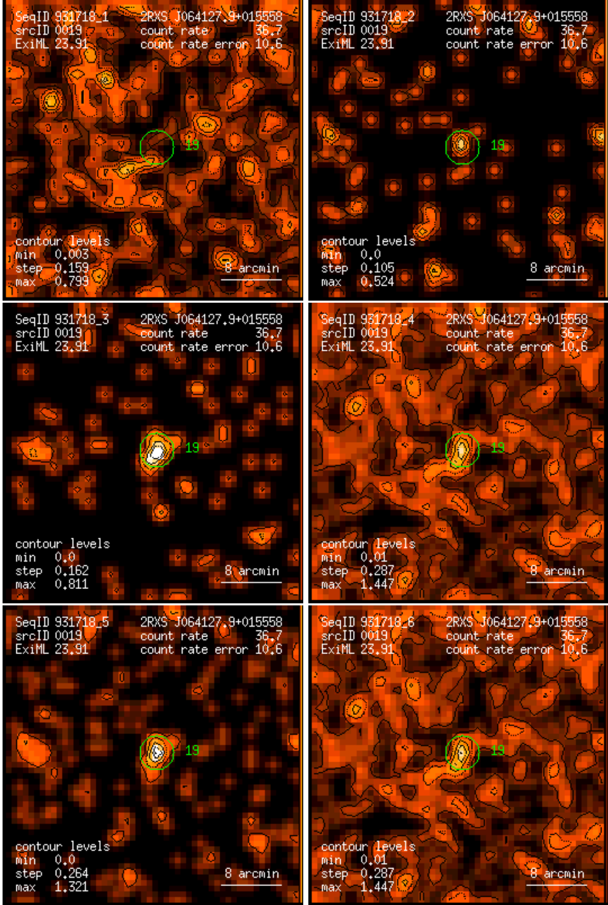
Figure 19: RASS 931718: detection 0019: band rate images, Gaussian filter: (1) PSPC channels 11 – 41, (2) 52 – 90, (3) 91 – 201, (4) 11 – 235, (5) 52 – 201, (6) 11 – 201. Broad band rates in counts/ks. Band rate contour levels in counts/ks/arcmin 2 .
