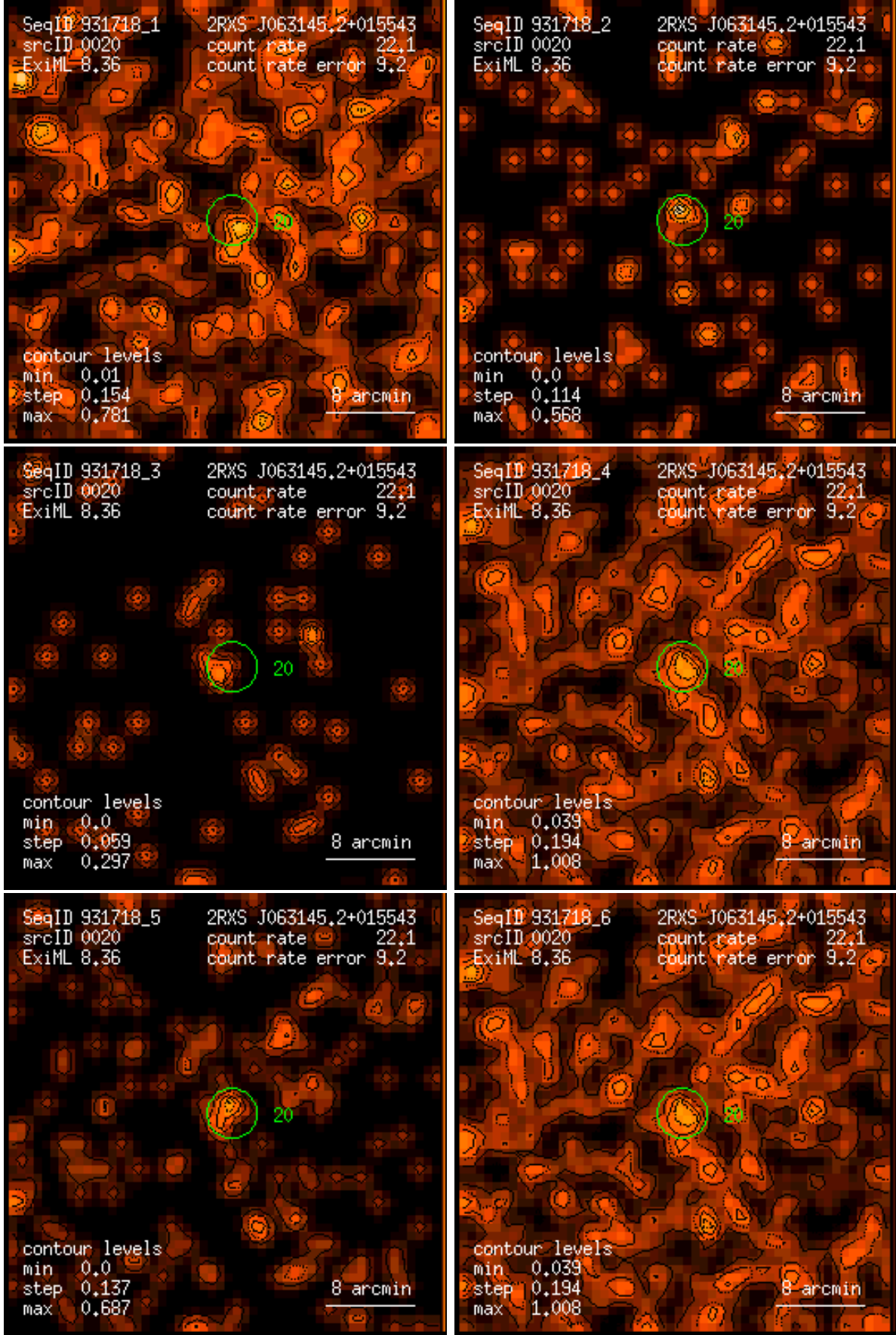
Figure 20: RASS 931718: detection 0020: band rate images, Gaussian filter: (1) PSPC channels 11 – 41, (2) 52 – 90, (3) 91 – 201, (4) 11 – 235, (5) 52 – 201, (6) 11 – 201. Broad band rates in counts/ks. Band rate contour levels in counts/ks/arcmin 2 .
