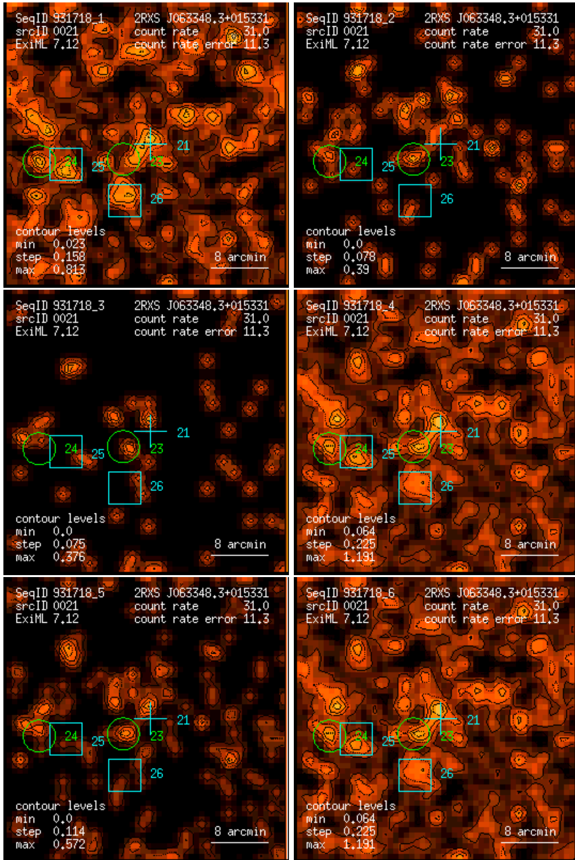
Figure 21: RASS 931718: detection 0021: band rate images, Gaussian filter: (1) PSPC channels 11 – 41, (2) 52 – 90, (3) 91 – 201, (4) 11 – 235, (5) 52 – 201, (6) 11 – 201. Broad band rates in counts/ks. Band rate contour levels in counts/ks/arcmin 2 .
