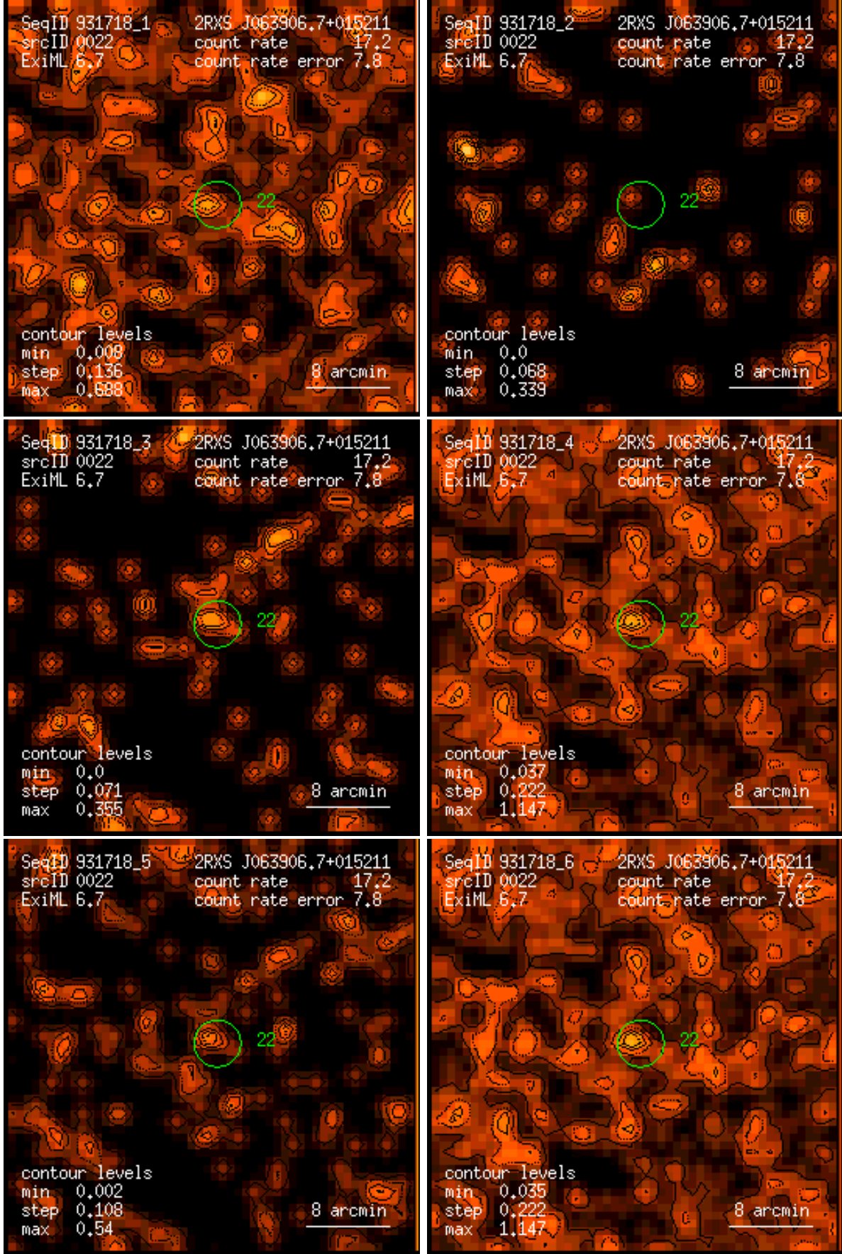
Figure 22: RASS 931718: detection 0022: band rate images, Gaussian filter: (1) PSPC channels 11 – 41, (2) 52 – 90, (3) 91 – 201, (4) 11 – 235, (5) 52 – 201, (6) 11 – 201. Broad band rates in counts/ks. Band rate contour levels in counts/ks/arcmin 2 .
