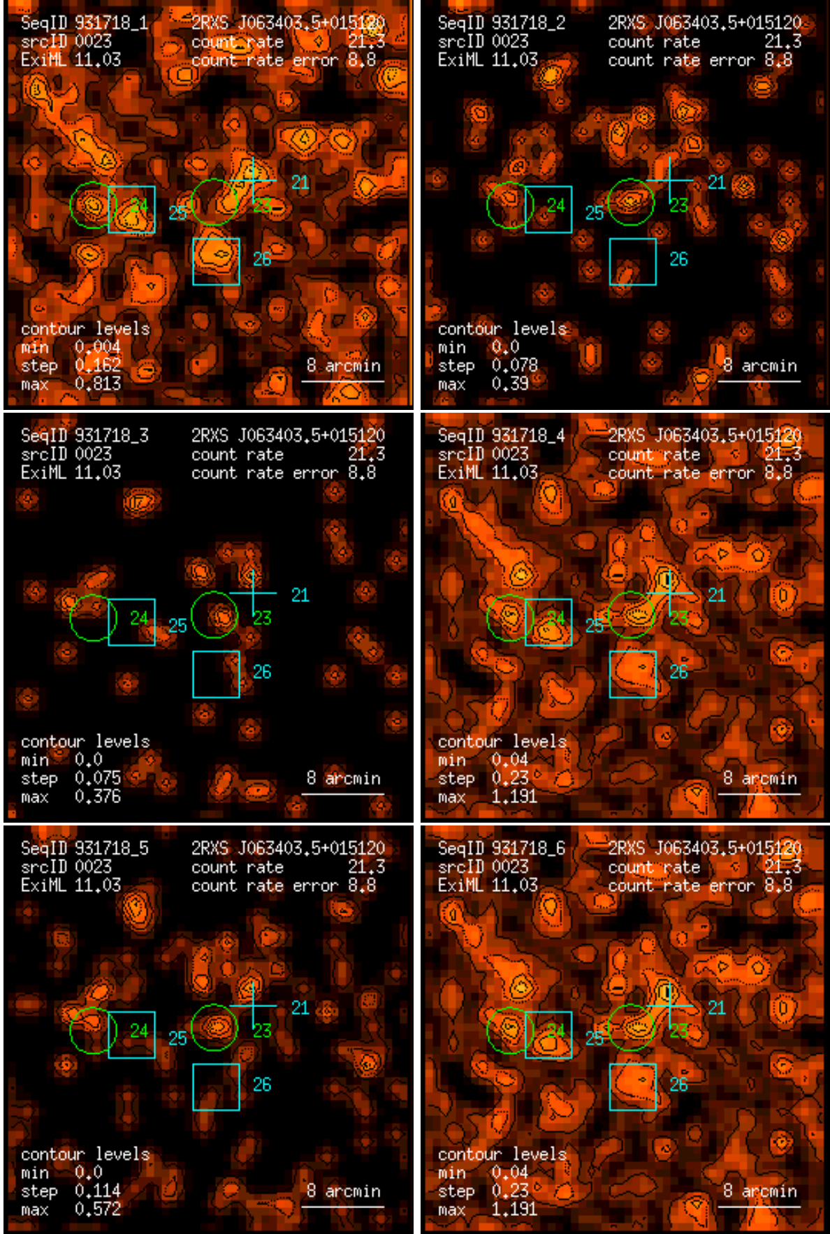
Figure 23: RASS 931718: detection 0023: band rate images, Gaussian filter: (1) PSPC channels 11 – 41, (2) 52 – 90, (3) 91 – 201, (4) 11 – 235, (5) 52 – 201, (6) 11 – 201. Broad band rates in counts/ks. Band rate contour levels in counts/ks/arcmin 2 .
