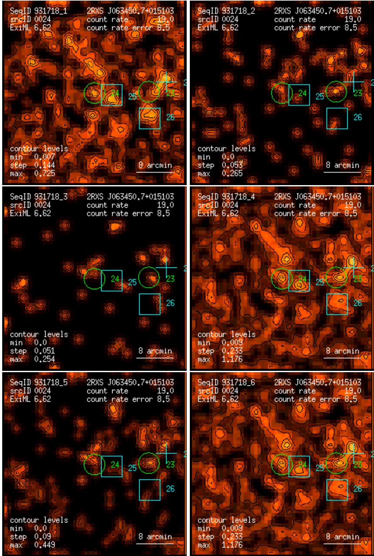
Figure 24: RASS 931718: detection 0024: band rate images, Gaussian filter: (1) PSPC channels 11 – 41, (2) 52 – 90, (3) 91 – 201, (4) 11 – 235, (5) 52 – 201, (6) 11 – 201. Broad band rates in counts/ks. Band rate contour levels in counts/ks/arcmin 2 .
