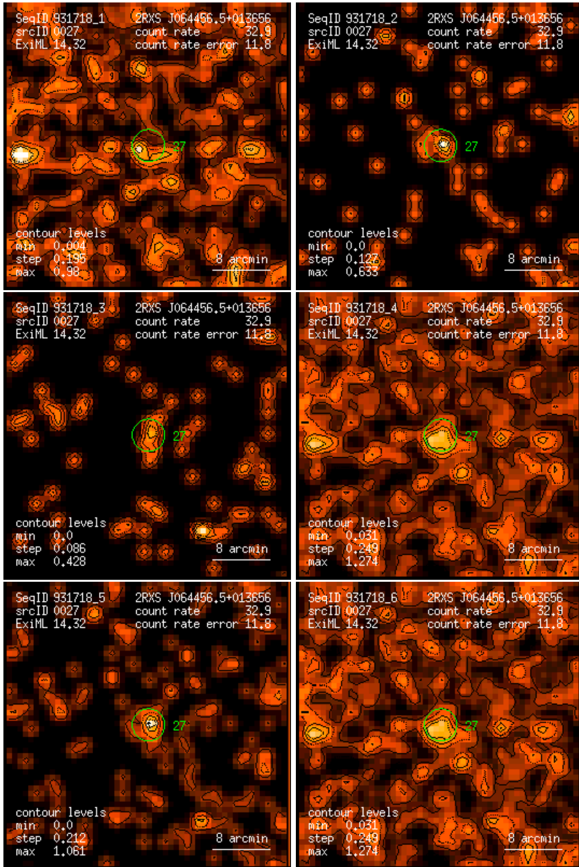
Figure 27: RASS 931718: detection 0027: band rate images, Gaussian filter: (1) PSPC channels 11 – 41, (2) 52 – 90, (3) 91 – 201, (4) 11 – 235, (5) 52 – 201, (6) 11 – 201. Broad band rates in counts/ks. Band rate contour levels in counts/ks/arcmin 2 .
