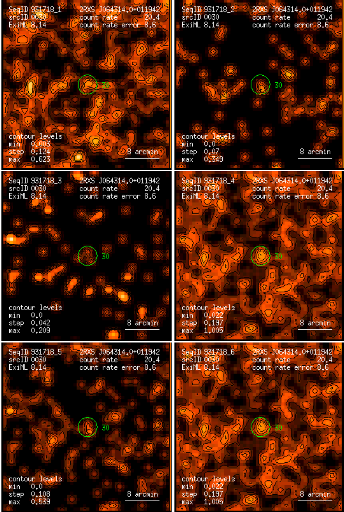
Figure 30: RASS 931718: detection 0030: band rate images, Gaussian filter: (1) PSPC channels 11 – 41, (2) 52 – 90, (3) 91 – 201, (4) 11 – 235, (5) 52 – 201, (6) 11 – 201. Broad band rates in counts/ks. Band rate contour levels in counts/ks/arcmin 2 .
