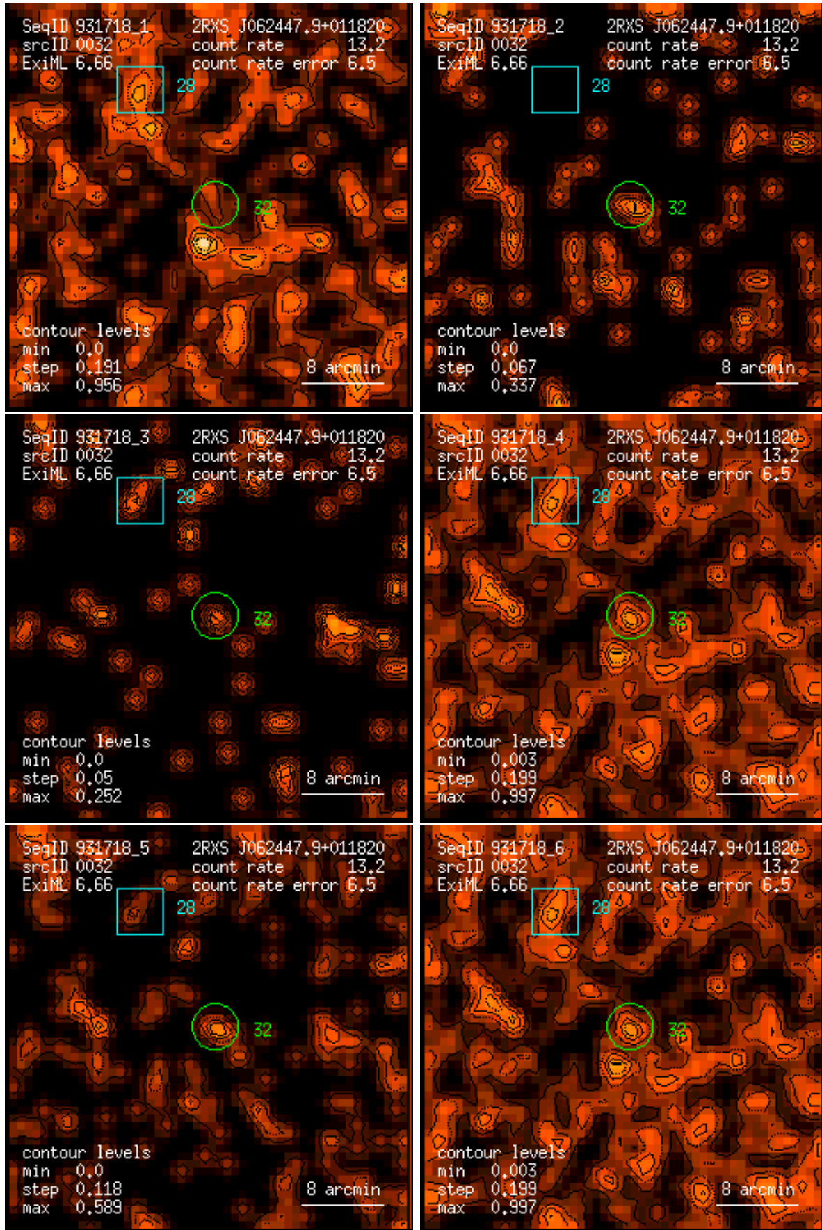
Figure 32: RASS 931718: detection 0032: band rate images, Gaussian filter: (1) PSPC channels 11 – 41, (2) 52 – 90, (3) 91 – 201, (4) 11 – 235, (5) 52 – 201, (6) 11 – 201. Broad band rates in counts/ks. Band rate contour levels in counts/ks/arcmin 2 .
