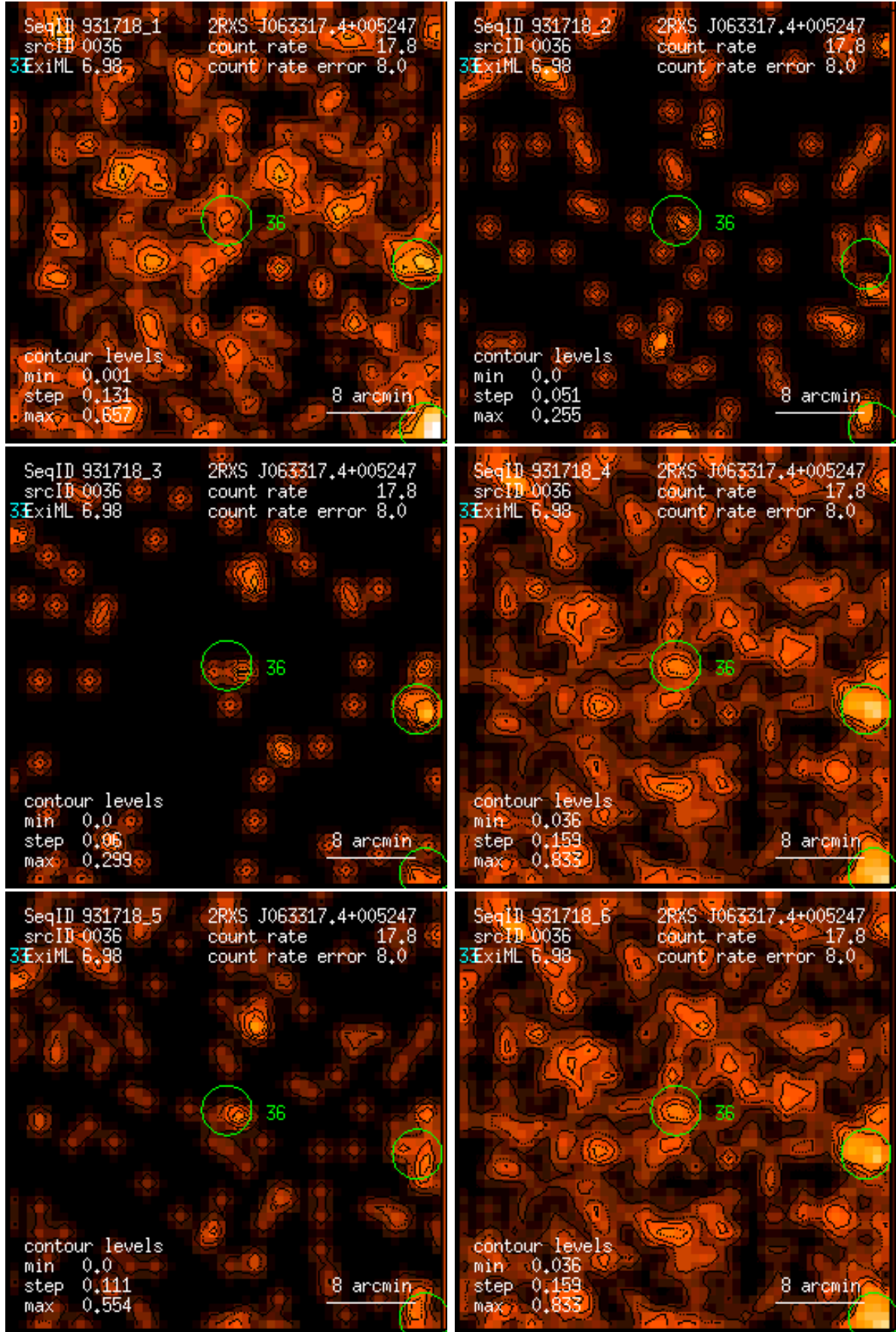
Figure 36: RASS 931718: detection 0036: band rate images, Gaussian filter: (1) PSPC channels 11 – 41, (2) 52 – 90, (3) 91 – 201, (4) 11 – 235, (5) 52 – 201, (6) 11 – 201. Broad band rates in counts/ks. Band rate contour levels in counts/ks/arcmin 2 .
