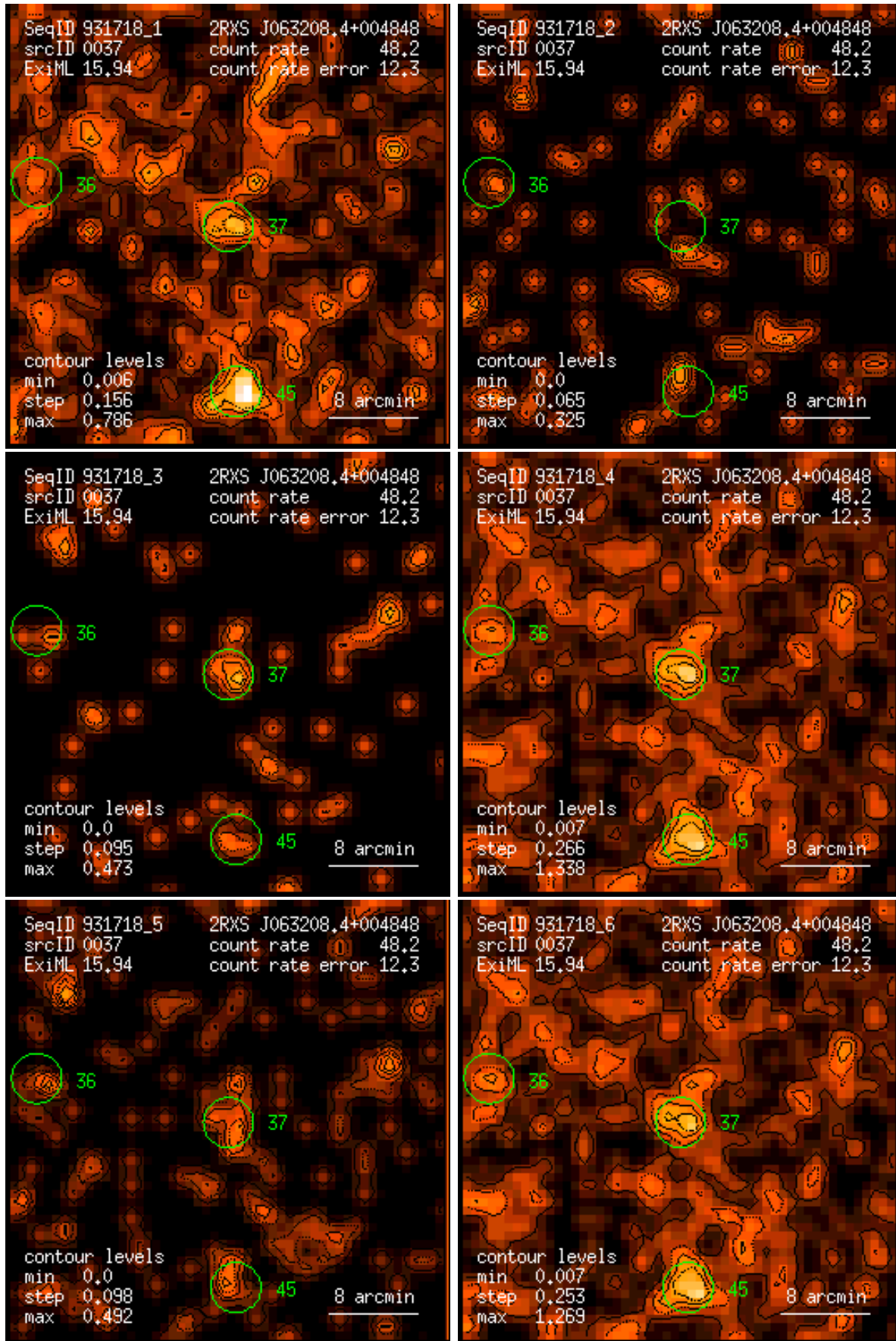
Figure 37: RASS 931718: detection 0037: band rate images, Gaussian filter: (1) PSPC channels 11 – 41, (2) 52 – 90, (3) 91 – 201, (4) 11 – 235, (5) 52 – 201, (6) 11 – 201. Broad band rates in counts/ks. Band rate contour levels in counts/ks/arcmin 2 .
