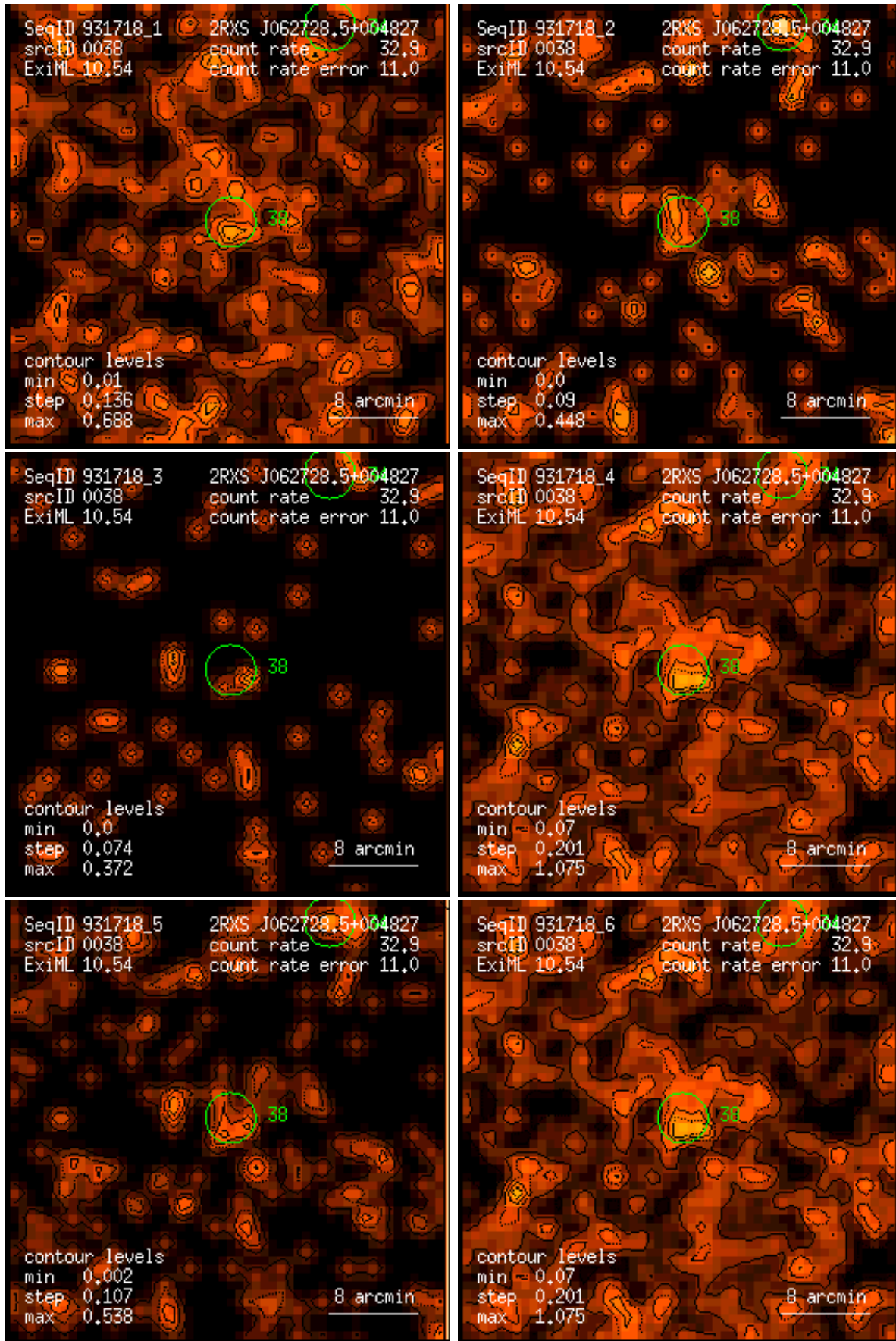
Figure 38: RASS 931718: detection 0038: band rate images, Gaussian filter: (1) PSPC channels 11 – 41, (2) 52 – 90, (3) 91 – 201, (4) 11 – 235, (5) 52 – 201, (6) 11 – 201. Broad band rates in counts/ks. Band rate contour levels in counts/ks/arcmin 2 .
