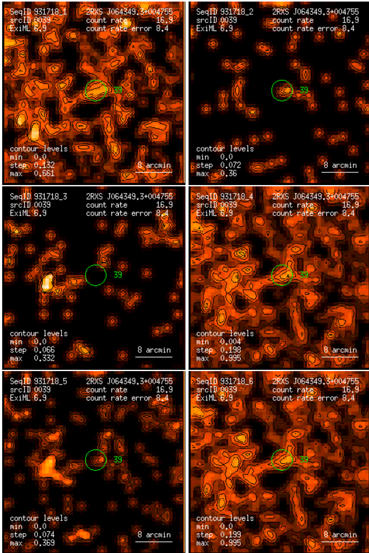
Figure 39: RASS 931718: detection 0039: band rate images, Gaussian filter: (1) PSPC channels 11 – 41, (2) 52 – 90, (3) 91 – 201, (4) 11 – 235, (5) 52 – 201, (6) 11 – 201. Broad band rates in counts/ks. Band rate contour levels in counts/ks/arcmin 2 .
