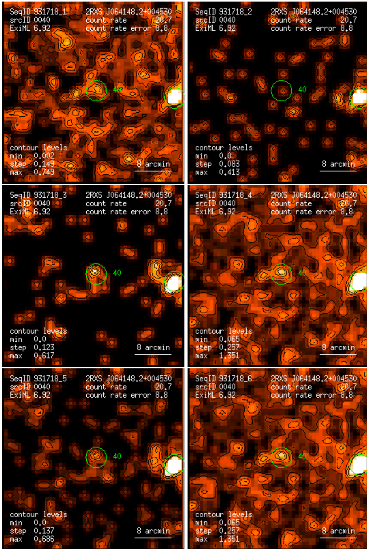
Figure 40: RASS 931718: detection 0040: band rate images, Gaussian filter: (1) PSPC channels 11 – 41, (2) 52 – 90, (3) 91 – 201, (4) 11 – 235, (5) 52 – 201, (6) 11 – 201. Broad band rates in counts/ks. Band rate contour levels in counts/ks/arcmin 2 .
