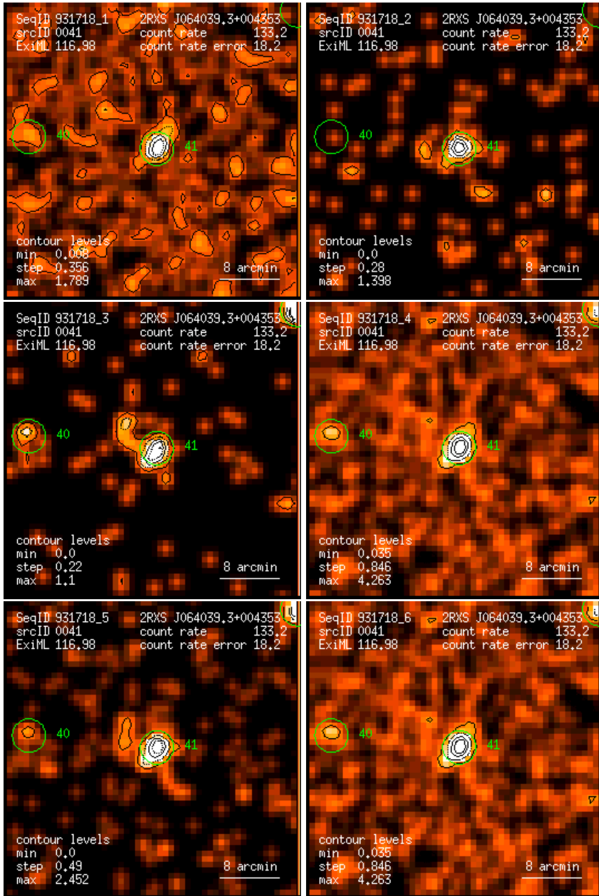
Figure 41: RASS 931718: detection 0041: band rate images, Gaussian filter: (1) PSPC channels 11 – 41, (2) 52 – 90, (3) 91 – 201, (4) 11 – 235, (5) 52 – 201, (6) 11 – 201. Broad band rates in counts/ks. Band rate contour levels in counts/ks/arcmin 2 .
