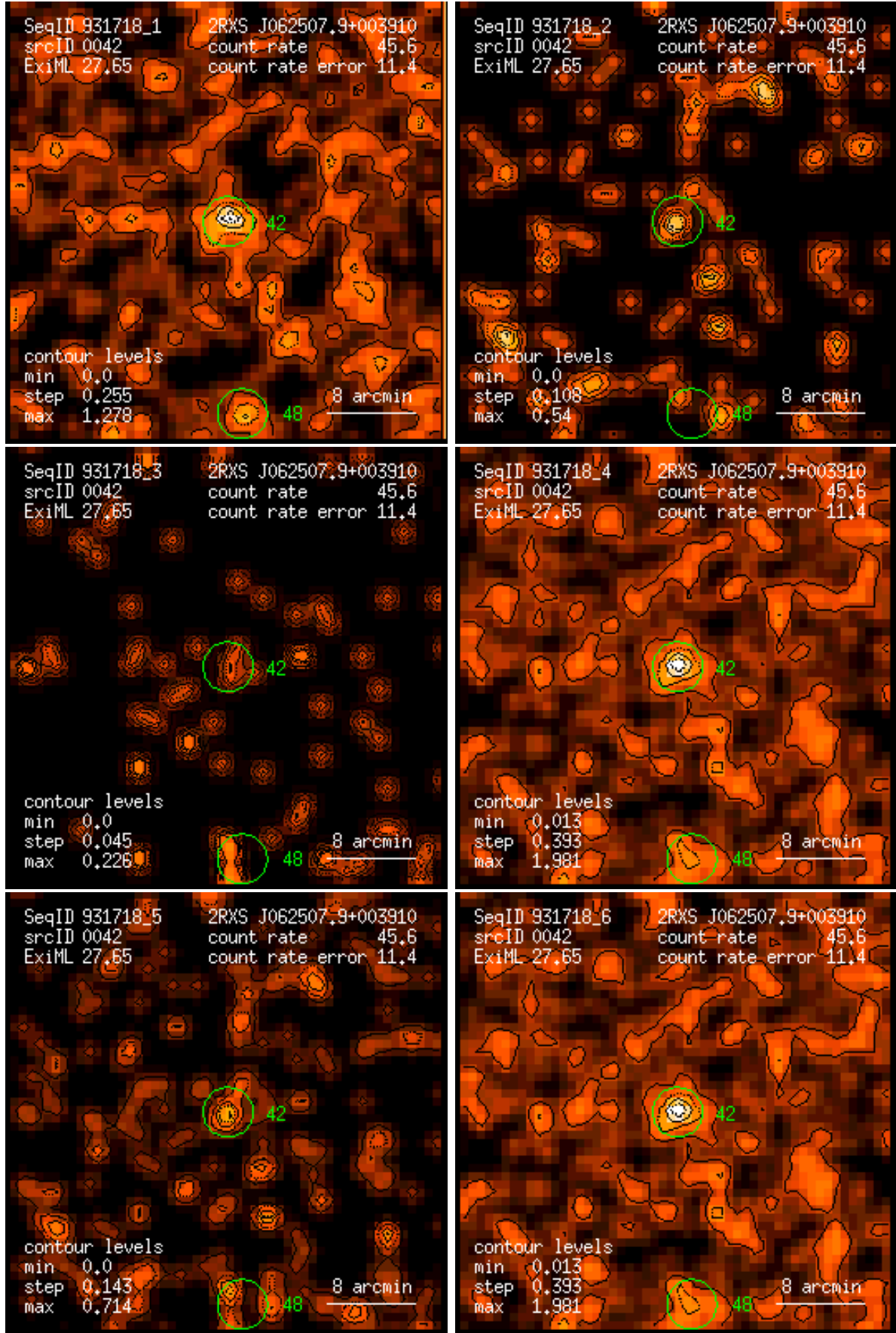
Figure 42: RASS 931718: detection 0042: band rate images, Gaussian filter: (1) PSPC channels 11 – 41, (2) 52 – 90, (3) 91 – 201, (4) 11 – 235, (5) 52 – 201, (6) 11 – 201. Broad band rates in counts/ks. Band rate contour levels in counts/ks/arcmin 2 .
