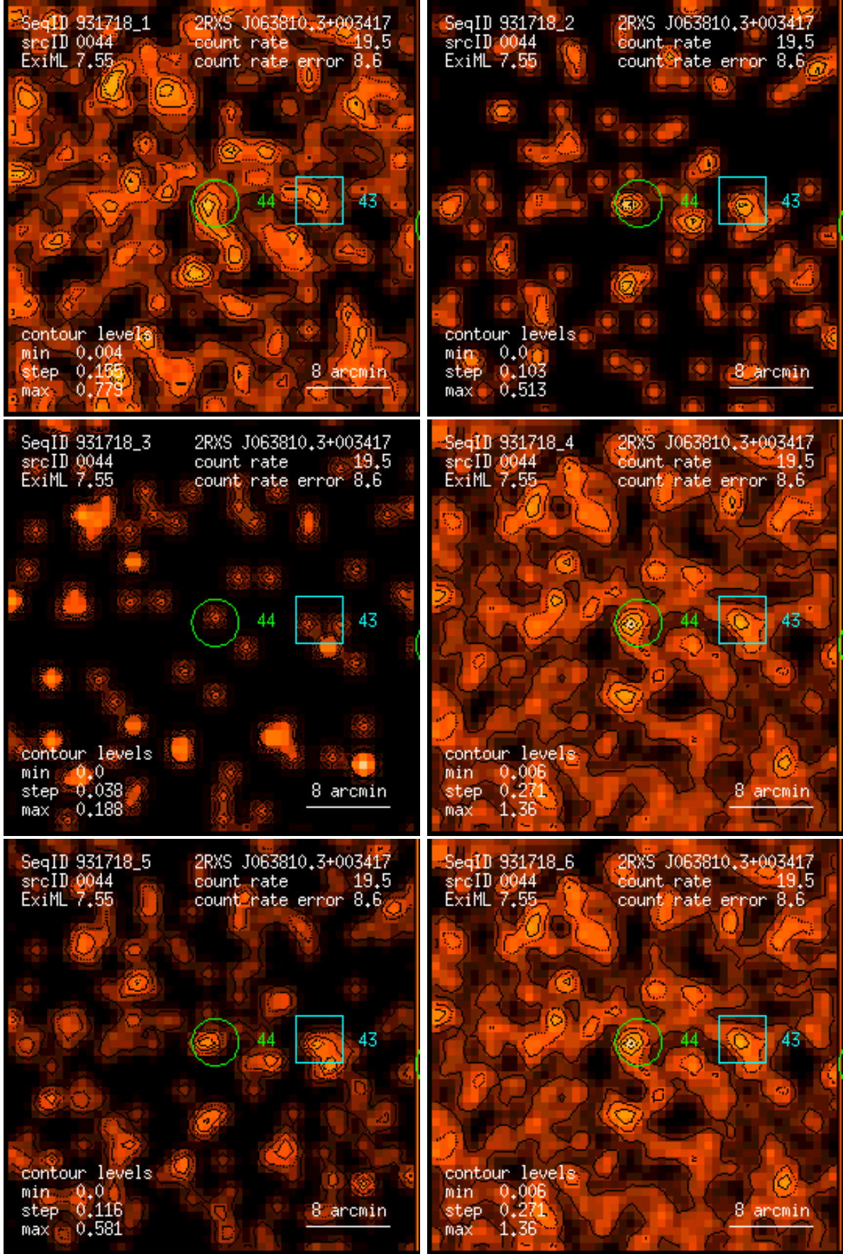
Figure 44: RASS 931718: detection 0044: band rate images, Gaussian filter: (1) PSPC channels 11 – 41, (2) 52 – 90, (3) 91 – 201, (4) 11 – 235, (5) 52 – 201, (6) 11 – 201. Broad band rates in counts/ks. Band rate contour levels in counts/ks/arcmin 2 .
