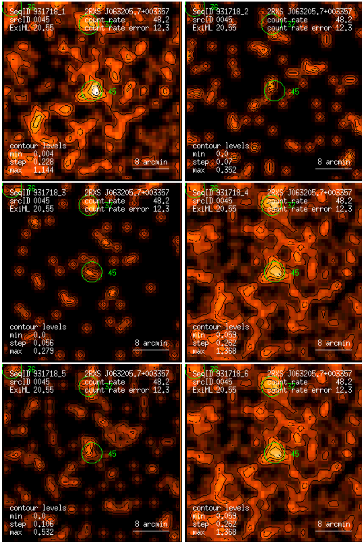
Figure 45: RASS 931718: detection 0045: band rate images, Gaussian filter: (1) PSPC channels 11 – 41, (2) 52 – 90, (3) 91 – 201, (4) 11 – 235, (5) 52 – 201, (6) 11 – 201. Broad band rates in counts/ks. Band rate contour levels in counts/ks/arcmin 2 .
