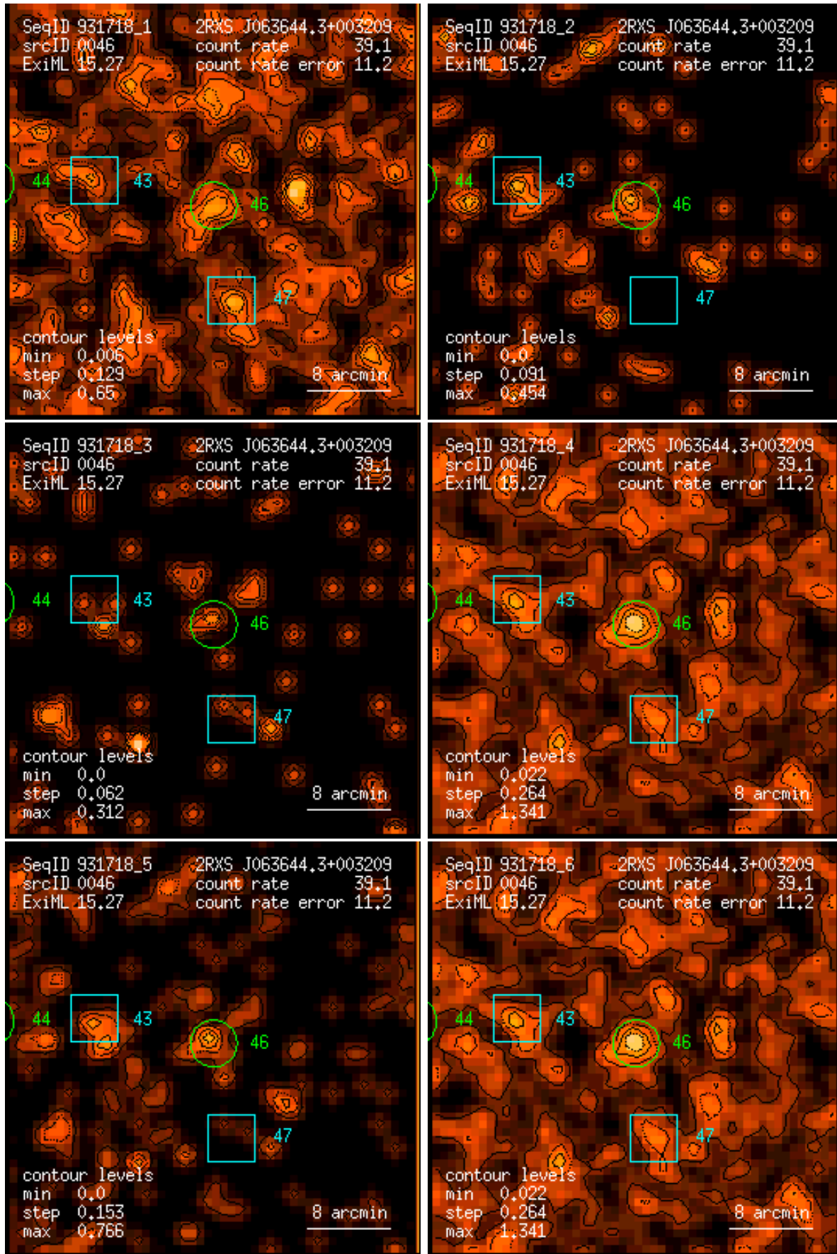
Figure 46: RASS 931718: detection 0046: band rate images, Gaussian filter: (1) PSPC channels 11 – 41, (2) 52 – 90, (3) 91 – 201, (4) 11 – 235, (5) 52 – 201, (6) 11 – 201. Broad band rates in counts/ks. Band rate contour levels in counts/ks/arcmin 2 .
