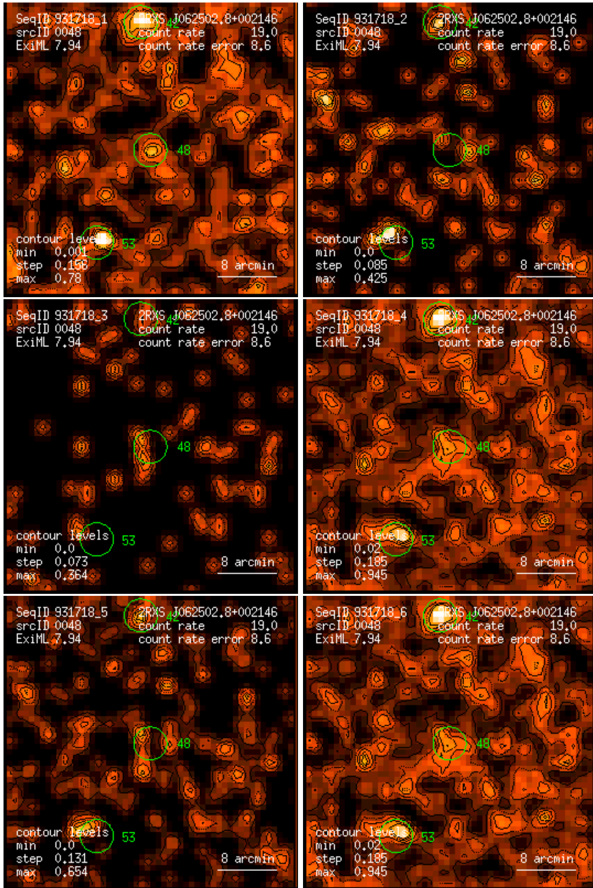
Figure 48: RASS 931718: detection 0048: band rate images, Gaussian filter: (1) PSPC channels 11 – 41, (2) 52 – 90, (3) 91 – 201, (4) 11 – 235, (5) 52 – 201, (6) 11 – 201. Broad band rates in counts/ks. Band rate contour levels in counts/ks/arcmin 2 .
