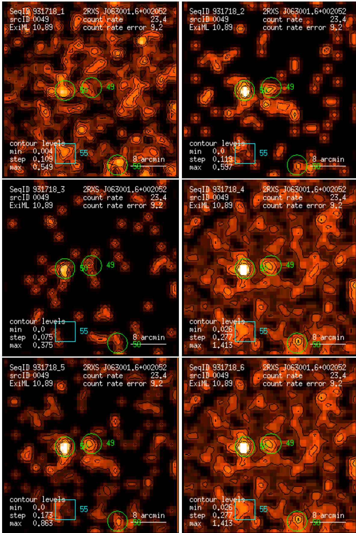
Figure 49: RASS 931718: detection 0049: band rate images, Gaussian filter: (1) PSPC channels 11 – 41, (2) 52 – 90, (3) 91 – 201, (4) 11 – 235, (5) 52 – 201, (6) 11 – 201. Broad band rates in counts/ks. Band rate contour levels in counts/ks/arcmin 2 .
