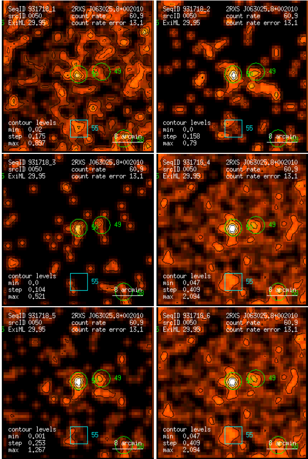
Figure 50: RASS 931718: detection 0050: band rate images, Gaussian filter: (1) PSPC channels 11 – 41, (2) 52 – 90, (3) 91 – 201, (4) 11 – 235, (5) 52 – 201, (6) 11 – 201. Broad band rates in counts/ks. Band rate contour levels in counts/ks/arcmin 2 .
