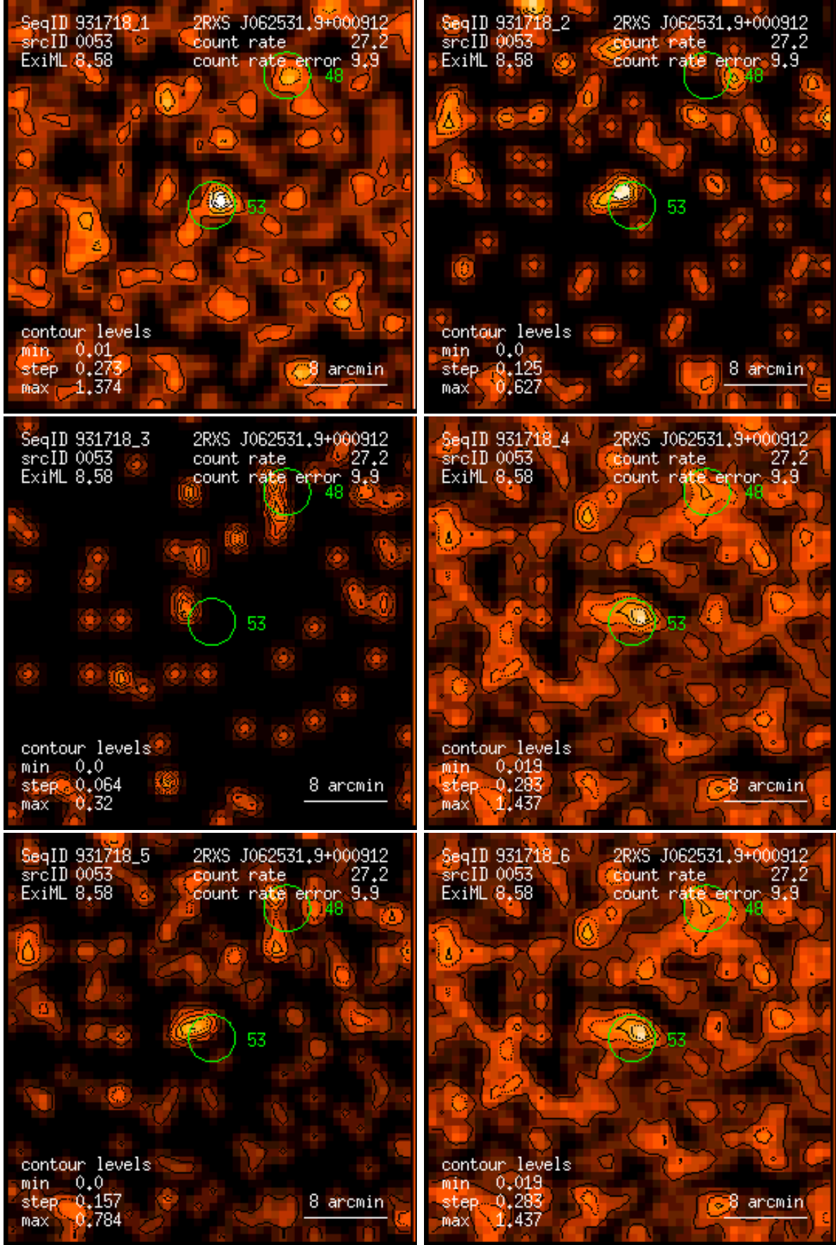
Figure 53: RASS 931718: detection 0053: band rate images, Gaussian filter: (1) PSPC channels 11 – 41, (2) 52 – 90, (3) 91 – 201, (4) 11 – 235, (5) 52 – 201, (6) 11 – 201. Broad band rates in counts/ks. Band rate contour levels in counts/ks/arcmin 2 .
