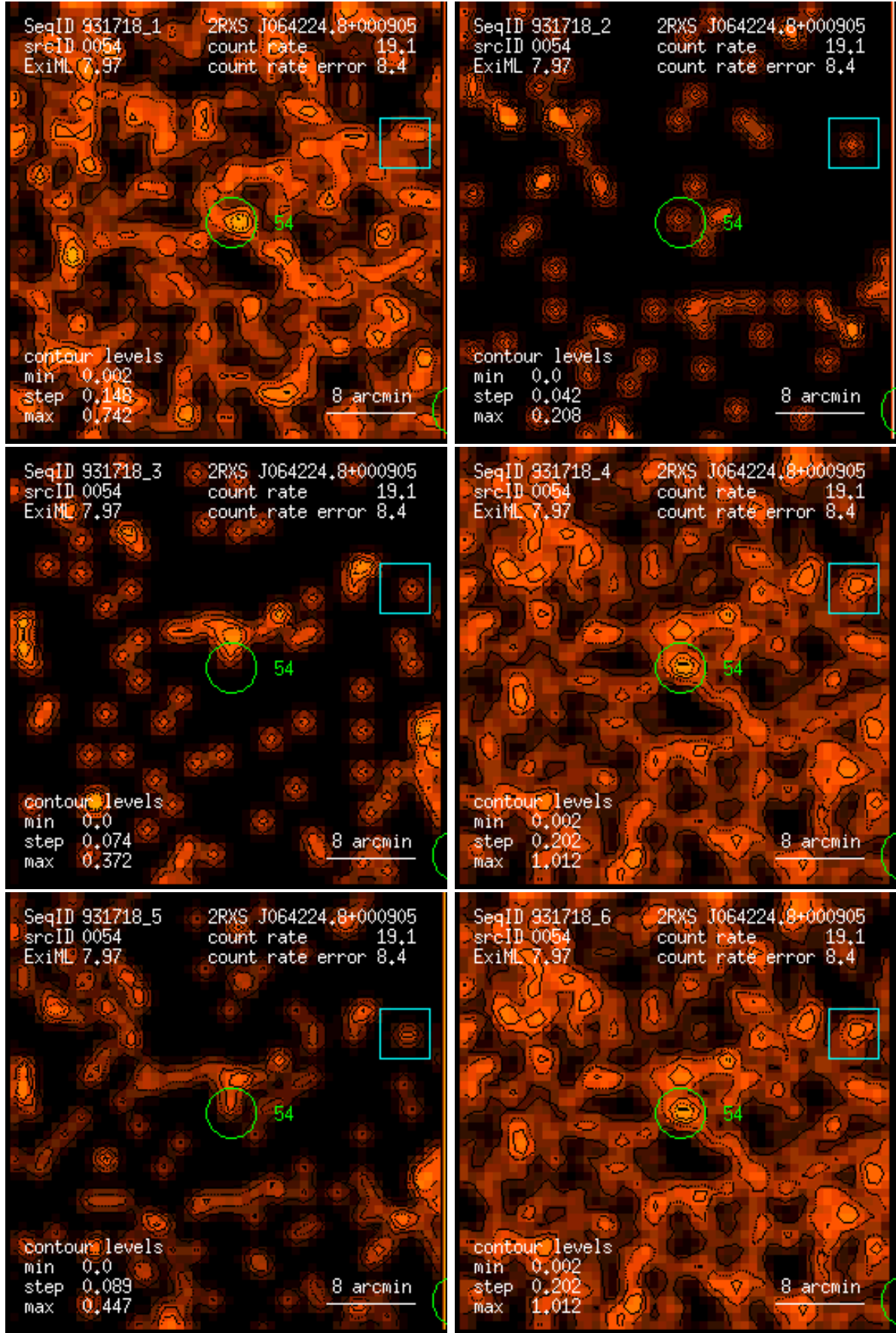
Figure 54: RASS 931718: detection 0054: band rate images, Gaussian filter: (1) PSPC channels 11 – 41, (2) 52 – 90, (3) 91 – 201, (4) 11 – 235, (5) 52 – 201, (6) 11 – 201. Broad band rates in counts/ks. Band rate contour levels in counts/ks/arcmin 2 .
