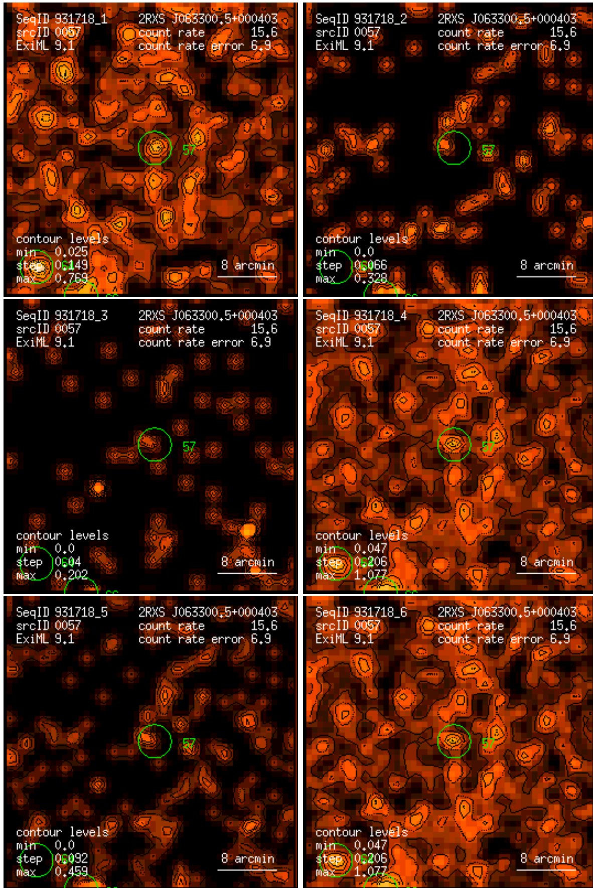
Figure 57: RASS 931718: detection 0057: band rate images, Gaussian filter: (1) PSPC channels 11 – 41, (2) 52 – 90, (3) 91 – 201, (4) 11 – 235, (5) 52 – 201, (6) 11 – 201. Broad band rates in counts/ks. Band rate contour levels in counts/ks/arcmin 2 .
