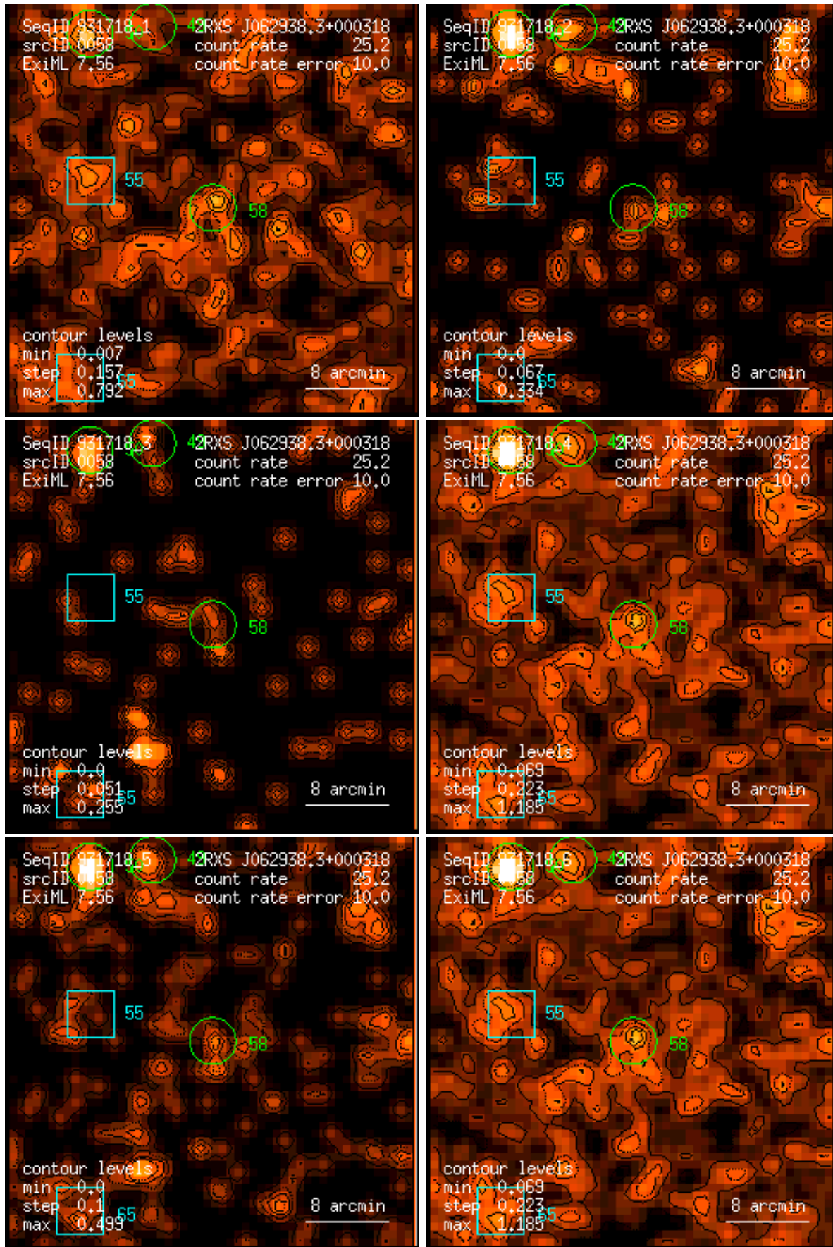
Figure 58: RASS 931718: detection 0058: band rate images, Gaussian filter: (1) PSPC channels 11 – 41, (2) 52 – 90, (3) 91 – 201, (4) 11 – 235, (5) 52 – 201, (6) 11 – 201. Broad band rates in counts/ks. Band rate contour levels in counts/ks/arcmin 2 .
