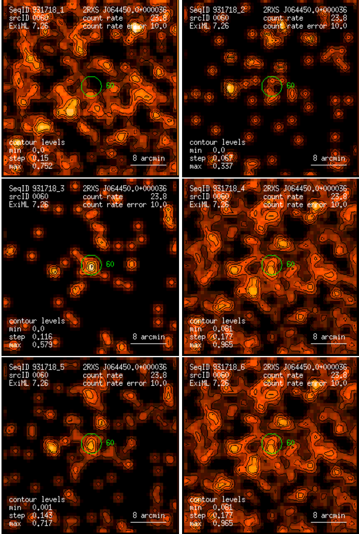
Figure 60: RASS 931718: detection 0060: band rate images, Gaussian filter: (1) PSPC channels 11 – 41, (2) 52 – 90, (3) 91 – 201, (4) 11 – 235, (5) 52 – 201, (6) 11 – 201. Broad band rates in counts/ks. Band rate contour levels in counts/ks/arcmin 2 .
