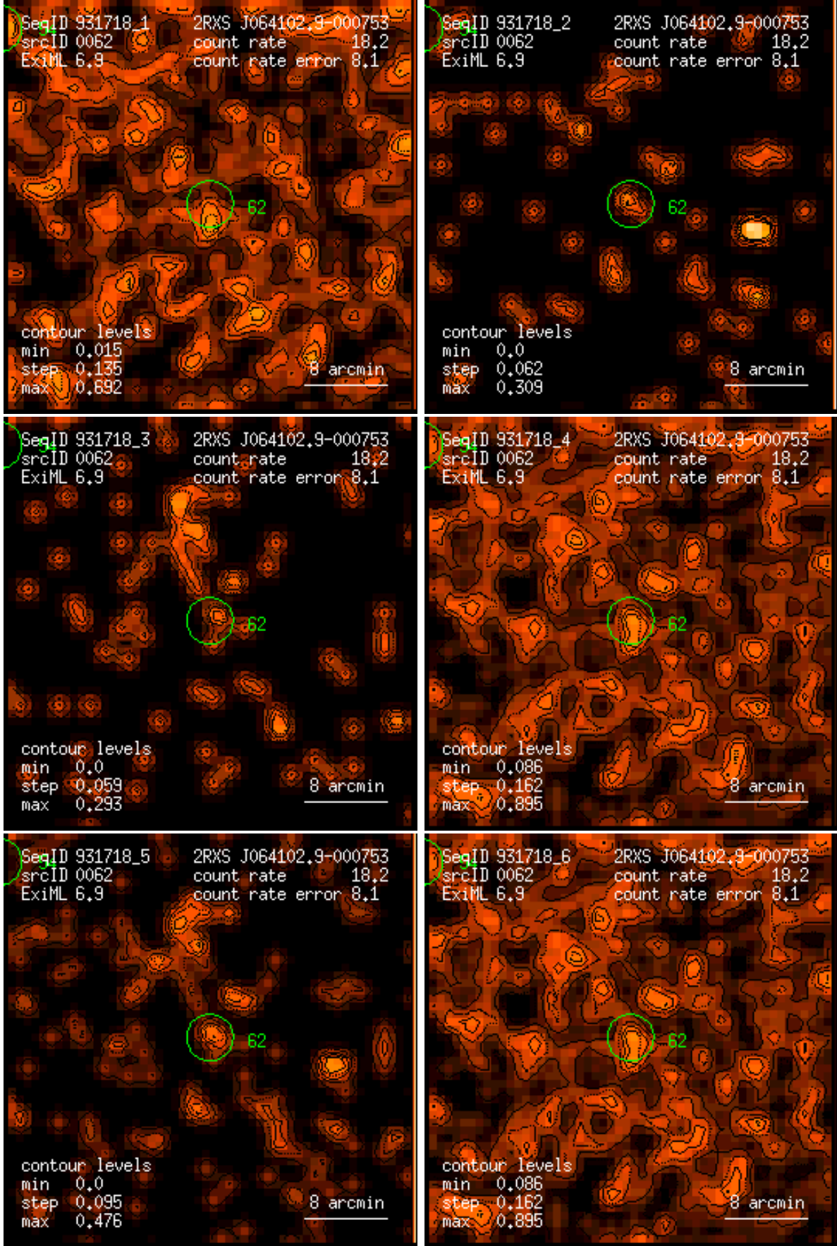
Figure 62: RASS 931718: detection 0062: band rate images, Gaussian filter: (1) PSPC channels 11 – 41, (2) 52 – 90, (3) 91 – 201, (4) 11 – 235, (5) 52 – 201, (6) 11 – 201. Broad band rates in counts/ks. Band rate contour levels in counts/ks/arcmin 2 .
