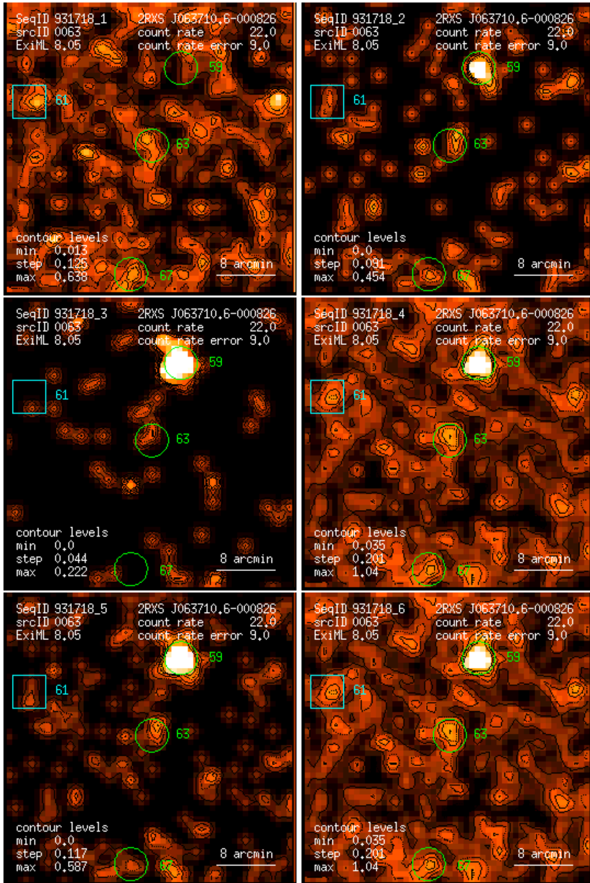
Figure 63: RASS 931718: detection 0063: band rate images, Gaussian filter: (1) PSPC channels 11 – 41, (2) 52 – 90, (3) 91 – 201, (4) 11 – 235, (5) 52 – 201, (6) 11 – 201. Broad band rates in counts/ks. Band rate contour levels in counts/ks/arcmin 2 .
