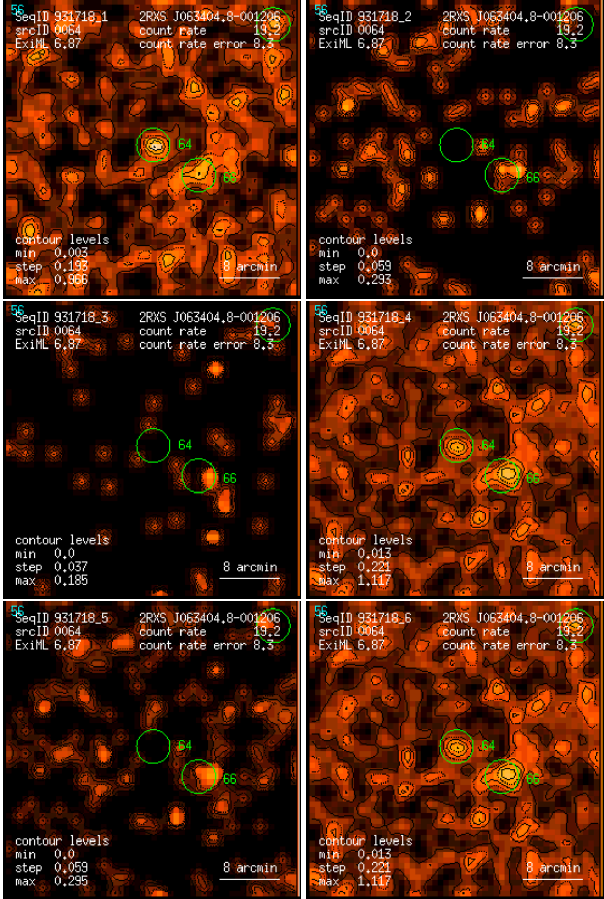
Figure 64: RASS 931718: detection 0064: band rate images, Gaussian filter: (1) PSPC channels 11 – 41, (2) 52 – 90, (3) 91 – 201, (4) 11 – 235, (5) 52 – 201, (6) 11 – 201. Broad band rates in counts/ks. Band rate contour levels in counts/ks/arcmin 2 .
