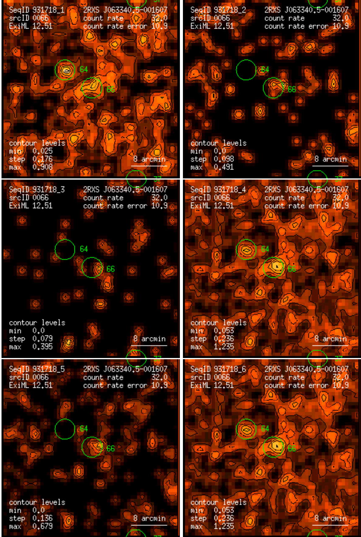
Figure 66: RASS 931718: detection 0066: band rate images, Gaussian filter: (1) PSPC channels 11 – 41, (2) 52 – 90, (3) 91 – 201, (4) 11 – 235, (5) 52 – 201, (6) 11 – 201. Broad band rates in counts/ks. Band rate contour levels in counts/ks/arcmin 2 .
