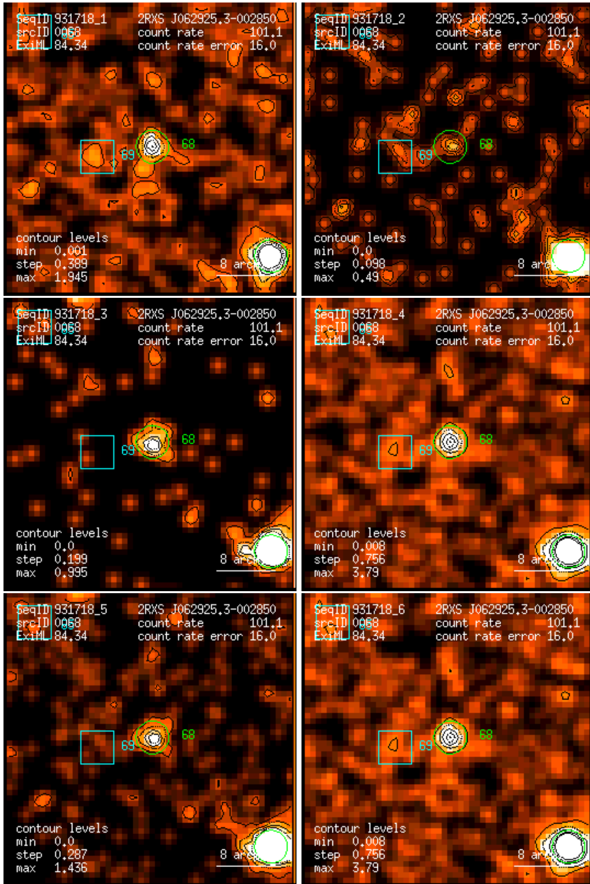
Figure 68: RASS 931718: detection 0068: band rate images, Gaussian filter: (1) PSPC channels 11 – 41, (2) 52 – 90, (3) 91 – 201, (4) 11 – 235, (5) 52 – 201, (6) 11 – 201. Broad band rates in counts/ks. Band rate contour levels in counts/ks/arcmin 2 .
