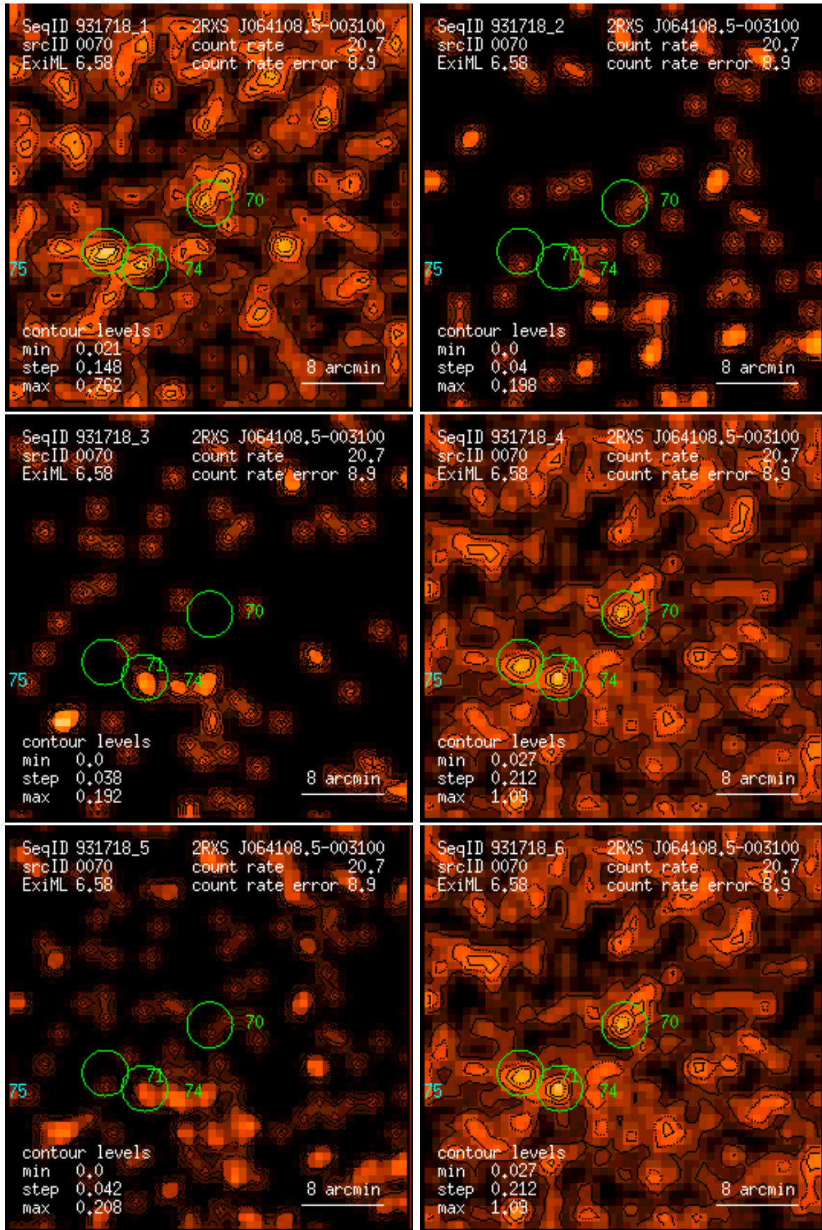
Figure 70: RASS 931718: detection 0070: band rate images, Gaussian filter: (1) PSPC channels 11 – 41, (2) 52 – 90, (3) 91 – 201, (4) 11 – 235, (5) 52 – 201, (6) 11 – 201. Broad band rates in counts/ks. Band rate contour levels in counts/ks/arcmin 2 .
