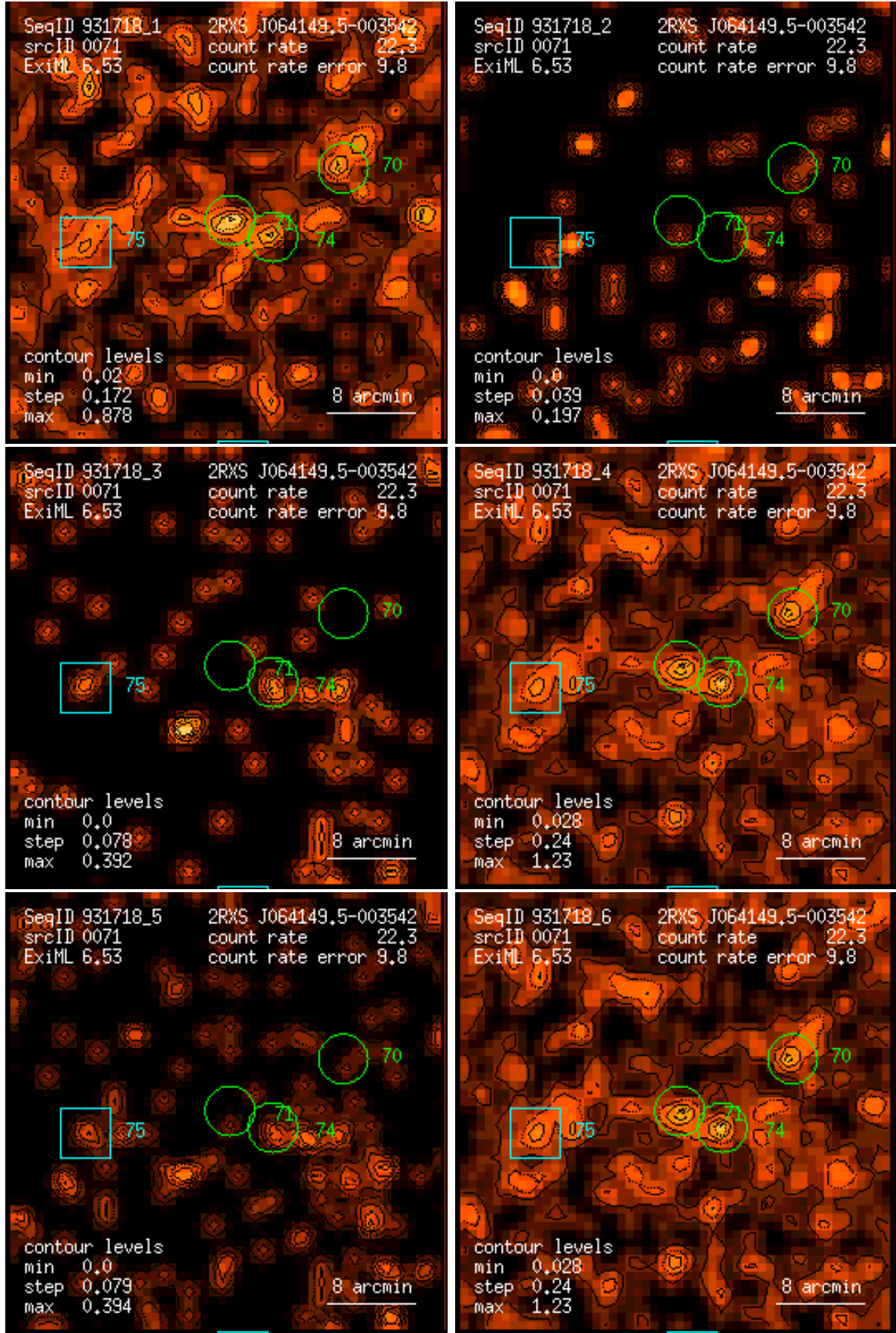
Figure 71: RASS 931718: detection 0071: band rate images, Gaussian filter: (1) PSPC channels 11 – 41, (2) 52 – 90, (3) 91 – 201, (4) 11 – 235, (5) 52 – 201, (6) 11 – 201. Broad band rates in counts/ks. Band rate contour levels in counts/ks/arcmin 2 .
