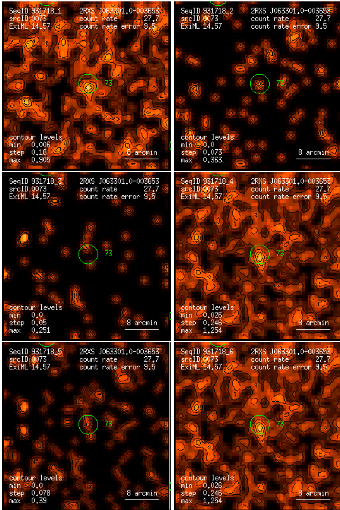
Figure 73: RASS 931718: detection 0073: band rate images, Gaussian filter: (1) PSPC channels 11 – 41, (2) 52 – 90, (3) 91 – 201, (4) 11 – 235, (5) 52 – 201, (6) 11 – 201. Broad band rates in counts/ks. Band rate contour levels in counts/ks/arcmin 2 .
