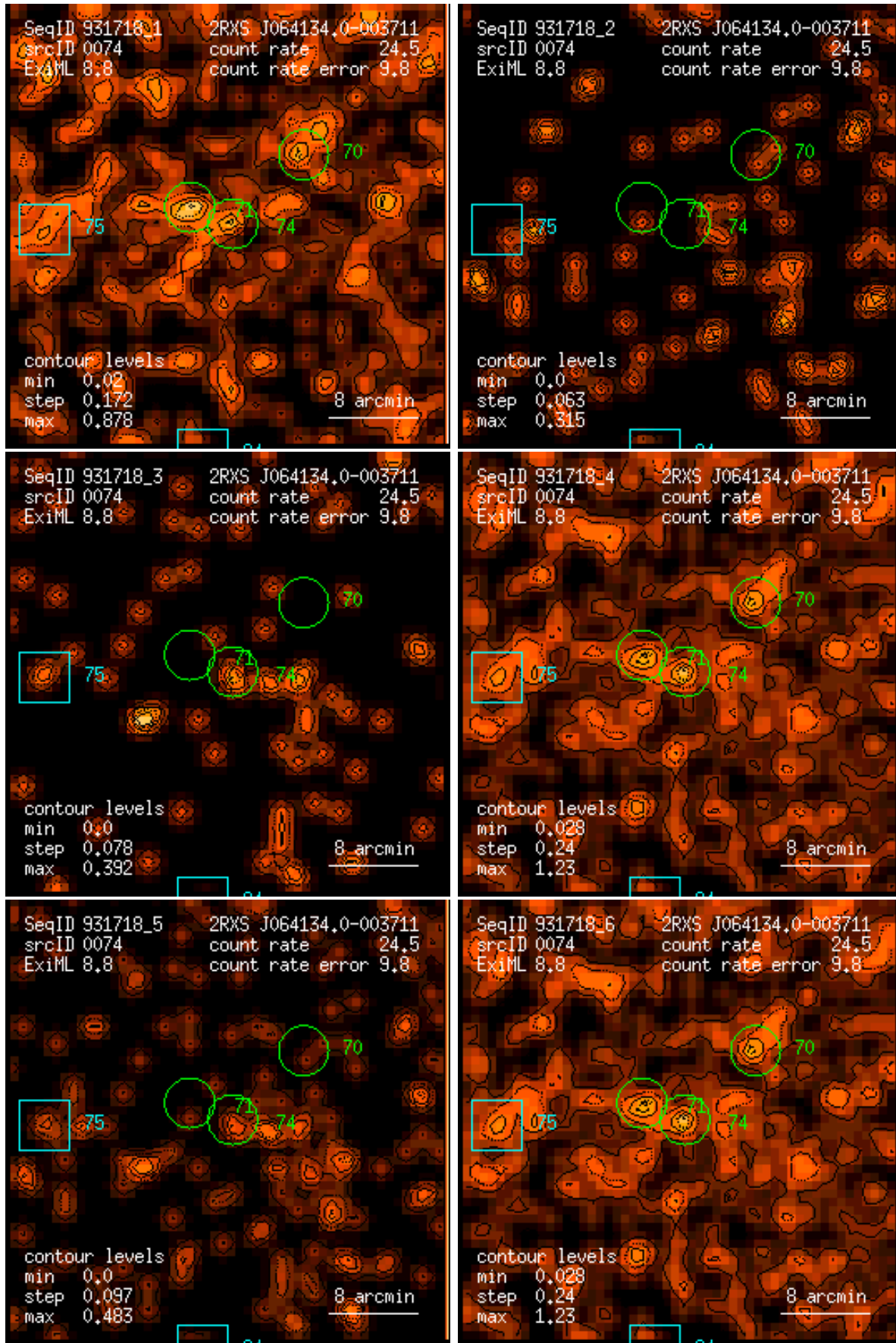
Figure 74: RASS 931718: detection 0074: band rate images, Gaussian filter: (1) PSPC channels 11 – 41, (2) 52 – 90, (3) 91 – 201, (4) 11 – 235, (5) 52 – 201, (6) 11 – 201. Broad band rates in counts/ks. Band rate contour levels in counts/ks/arcmin 2 .
