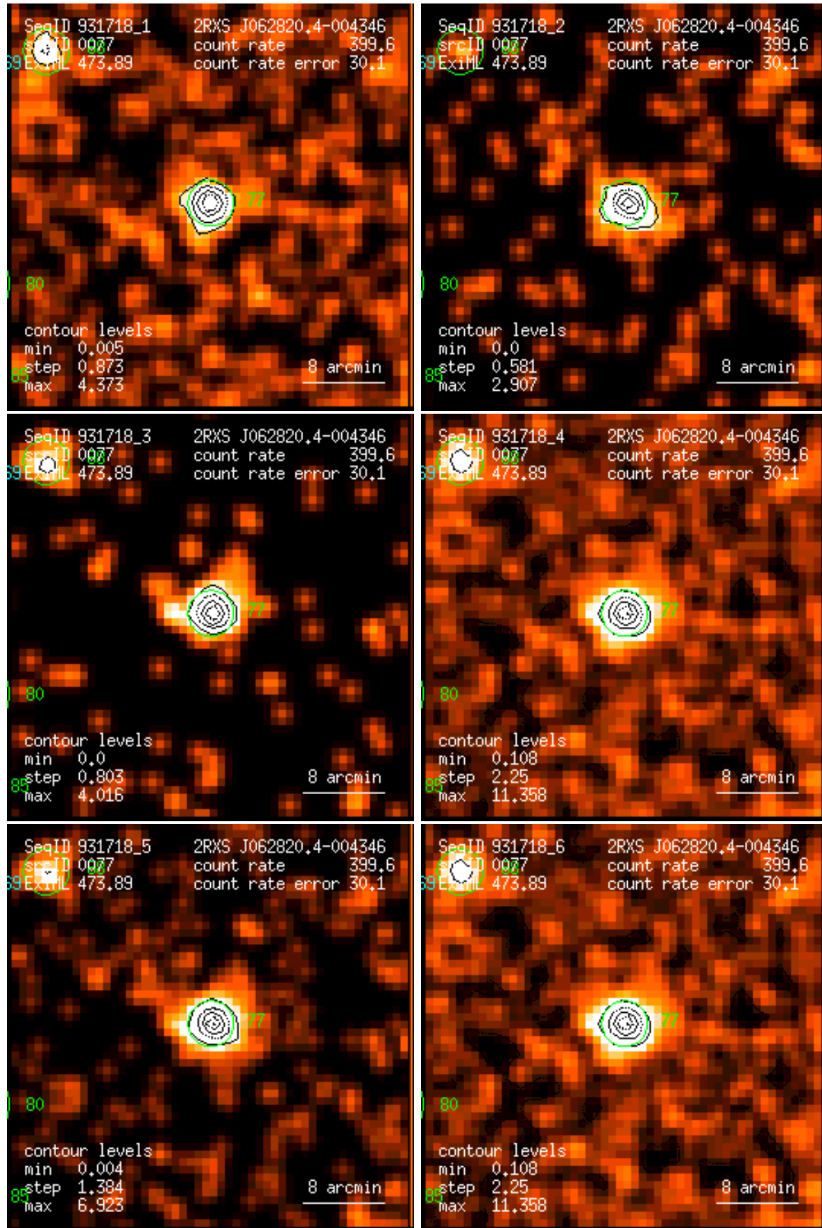
Figure 77: RASS 931718: detection 0077: band rate images, Gaussian filter: (1) PSPC channels 11 – 41, (2) 52 – 90, (3) 91 – 201, (4) 11 – 235, (5) 52 – 201, (6) 11 – 201. Broad band rates in counts/ks. Band rate contour levels in counts/ks/arcmin 2 .
