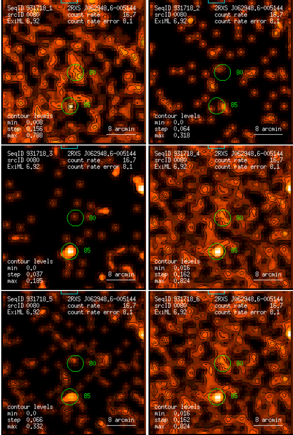
Figure 80: RASS 931718: detection 0080: band rate images, Gaussian filter: (1) PSPC channels 11 – 41, (2) 52 – 90, (3) 91 – 201, (4) 11 – 235, (5) 52 – 201, (6) 11 – 201. Broad band rates in counts/ks. Band rate contour levels in counts/ks/arcmin 2 .
