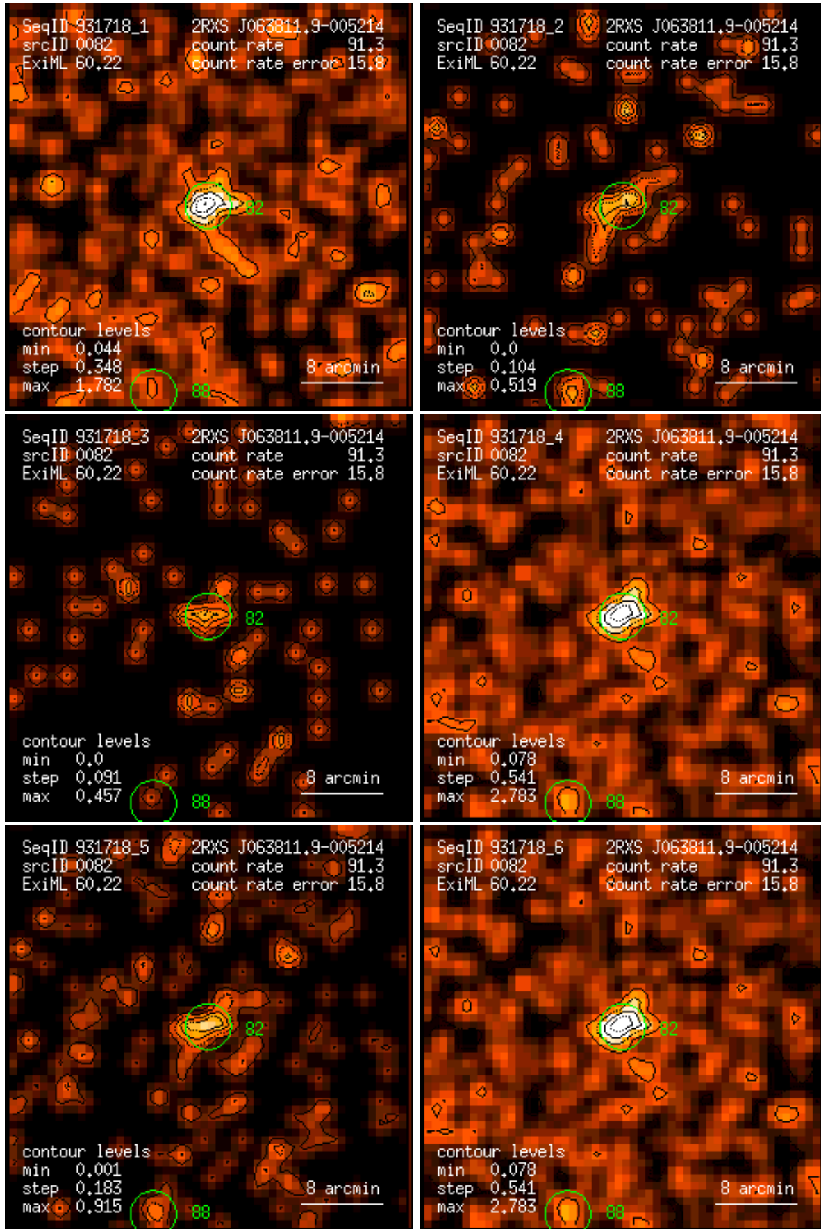
Figure 82: RASS 931718: detection 0082: band rate images, Gaussian filter: (1) PSPC channels 11 – 41, (2) 52 – 90, (3) 91 – 201, (4) 11 – 235, (5) 52 – 201, (6) 11 – 201. Broad band rates in counts/ks. Band rate contour levels in counts/ks/arcmin 2 .
