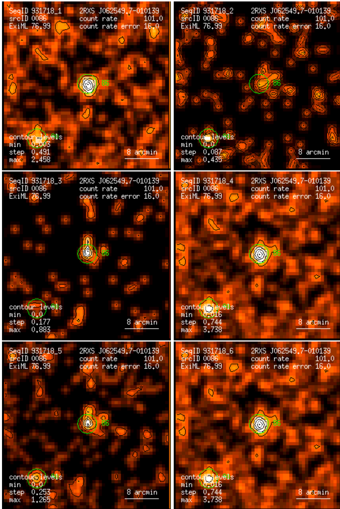
Figure 86: RASS 931718: detection 0086: band rate images, Gaussian filter: (1) PSPC channels 11 – 41, (2) 52 – 90, (3) 91 – 201, (4) 11 – 235, (5) 52 – 201, (6) 11 – 201. Broad band rates in counts/ks. Band rate contour levels in counts/ks/arcmin 2 .
